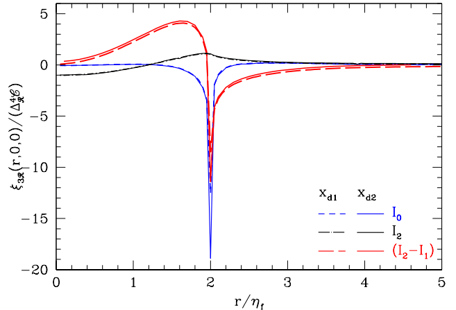
FIG. 13. Contribution to the real space three-point correlation function from the three terms in Eq. (A25). The thick dashed curves were computed for damping scale x_d = x_{d1} = 200 with an infrared cutoff at k_{\min} = 0.1/\eta_f , while the corresponding thin solid curves were calculated with x_{d2} = 1000 .
