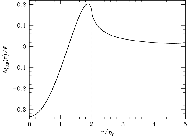
FIG. 11. Real space two-point correlation function changes due to the addition of a step feature ( d \rightarrow 0 ). At r/\eta_f = 2 , the slope of the correlation function diverges as the dashed line indicates.
