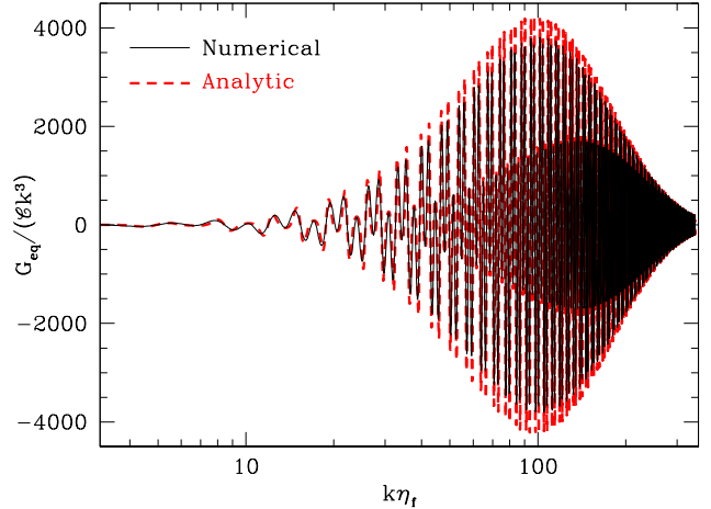
FIG. 4. Equilateral bispectrum computed using the analytic approximation in Eq. (48) (red dashed) compared with a full numerical evaluation of the integral in Eq. (45) for a large amplitude c \approx \epsilon_0/6 (or \mathcal{C}_0 = 1, \mathcal{C} = 2/3 ). Here the location, amplitude and damping scale of the feature have been nonlinearly scaled according to Eq. (33) and Eq. (35).
