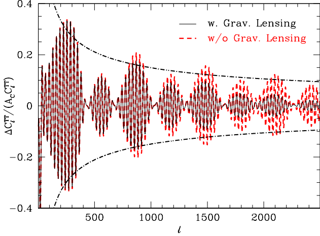
FIG. 5. Fractional difference of the temperature power spectrum of a model with \eta_f = 1.44 Gpc, c = 10^{-5} and d = 10^{-5} , relative to a model with c = 0 per unit power spectrum feature amplitude A_C (see Eq. 69). The case without gravitational lensing is shown in red dashed lines, and when gravitational lensing is taken into account is shown in black solid lines. In black dot-dashed lines we show the expected \ell^{-1/2} envelope from Eq. (70).
