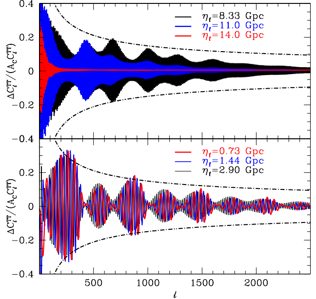
FIG. 6. Fractional difference of the temperature power spectrum (relative to a model with c = 0 ) of a model with c = 10^{-5} and d = 10^{-5} and different step positions. Gravitational lensing is taken into account in these examples. Note that as D/\eta_f \rightarrow 1 (in the upper panel), the nodes shift, and the shape changes significantly. In black dot-dashed lines we show the expected \ell^{-1/2} envelope from Eq. (70).
