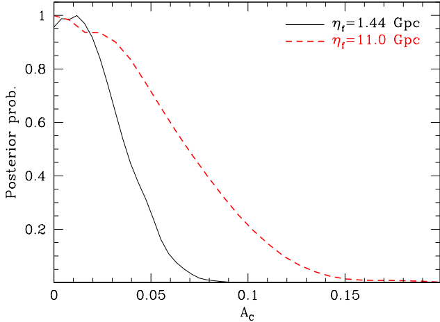
FIG. 7. Posterior probability distribution of the oscillation amplitude A_C in the angular power spectrum for representative value of \eta_f = 1.44 and 11 Gpc. The constraint weakens as \eta_f approaches the horizon for typical cases. For specific values of \eta_f the peak of the posterior is shifted to A_C \sim 0.1 with comparable distribution width (see text).
