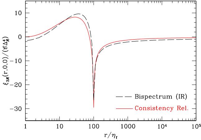
FIG. 15. The contribution to the real space three-point correlation function from the infra-red terms (the second two terms) in Eq. (A25) (dashed black curve) and the consistency relation of Eq. (A35) (red, solid). We take x_d = 100 with an infrared cutoff at k_{\min} = 0.001/\eta_f .
