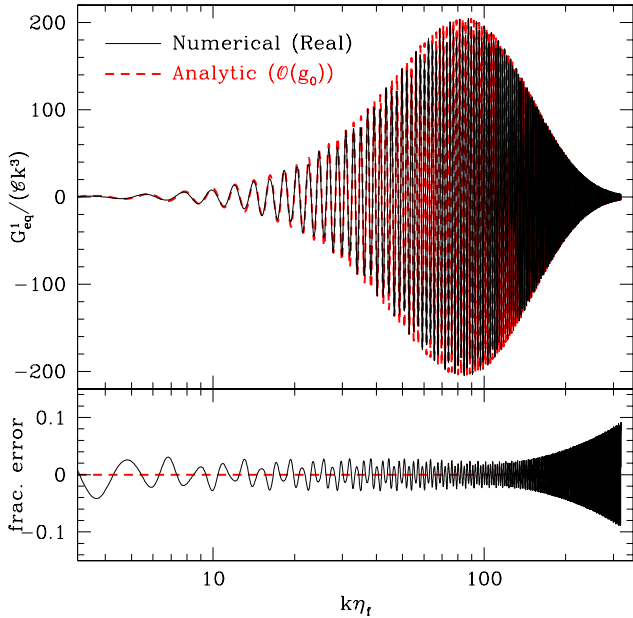
FIG. 16. First order corrections to the equilateral bispectrum computed using the analytic approximation Eq. (B11) and (B14) compared with the numerical evaluation of the second term in Eq. (B5) for a step with height c = 10^{-5} and width d = 0.001 . The lower panel here shows the fractional error of the full bispectrum, once this first order correction is taken into account.
