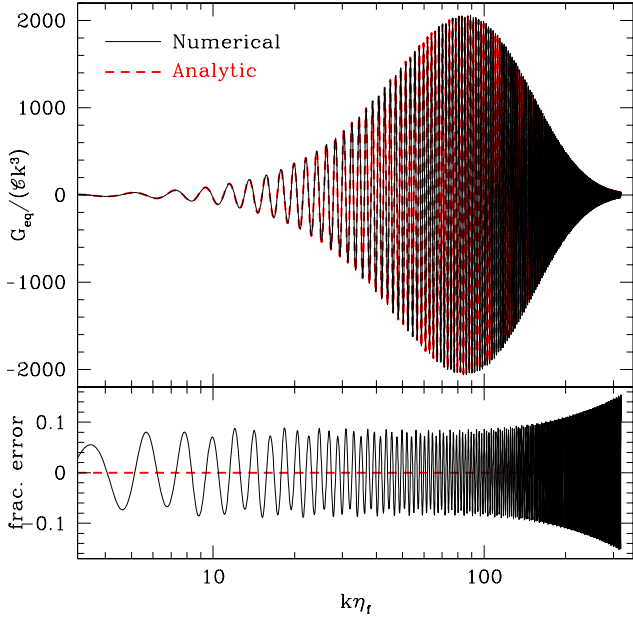
FIG. 3. Equilateral bispectrum computed using the analytic approximation in Eq. (48) (red dashed) compared with a full numerical evaluation of the integral in Eq. (45) for a small amplitude c = 10^{-5} (or \mathcal{C} \ll 1 ). The lower panel shows the difference between the curves, expressed as a fraction of the envelope of the analytic approximation in Eq. (63).
