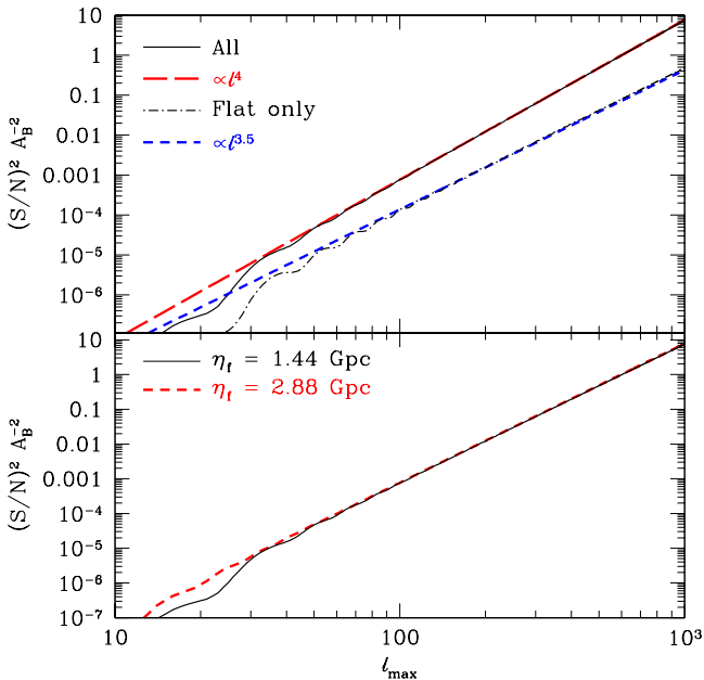
FIG. 9. The square of the SNR per unit bispectrum amplitude ( A_B ) for \ell_d = 8514 for all triangles, and for flat configurations only. We also plot the scaling relations from §VIC. In the lower panel, we demonstrate that changing \eta_f while fixing A_B and \ell_d leaves the SNR fixed at high \ell .
