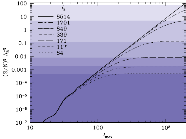
FIG. 10. The square of the SNR per unit bispectrum amplitude ( A_B ) for various damping scales \ell_d . The shaded regions indicate the prediction of our scaling formula in Eq. (96) and match the asymptotic high \ell \gg \ell_d saturation point for each case.
