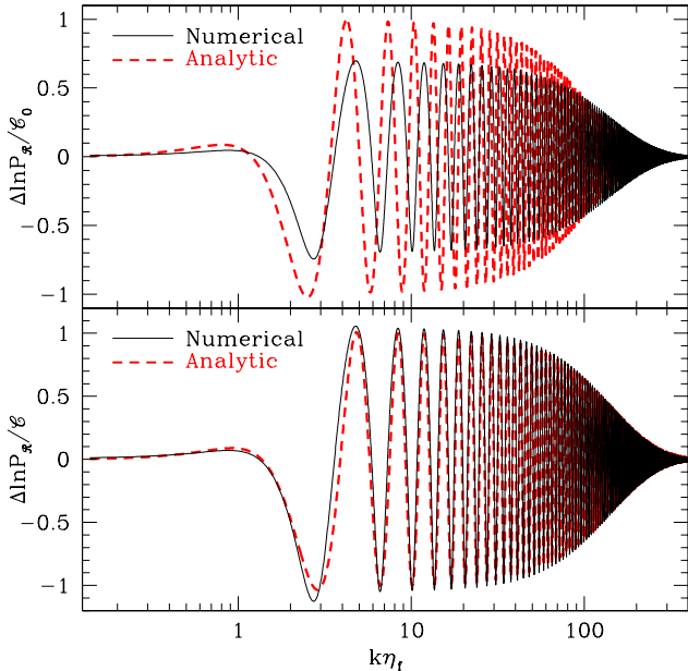
FIG. 2. Initial curvature power spectrum evaluated numerically (in solid black curves) compared with the approximation in Eq. (32) (in dashed red curves) for a large amplitude c = \epsilon_0/6 (or \mathcal{C}_0 = 1 , \mathcal{C} = 2/3 ), where the linear expansion is violated by order unity terms. Using the leading order expressions for the step location, oscillation amplitude and damping \eta_f , \mathcal{C} = \mathcal{C}_0 and x_d (upper panel) leads to phase and amplitude errors that are largely corrected by non-linearly rescaling these parameters using Eqs. (33) and (35) (lower panel).
