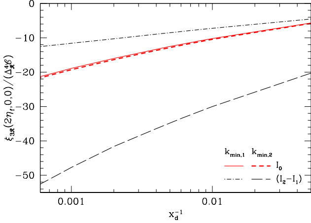
FIG. 14. Behavior of the various contributions to the real space three-point correlation function \xi_{3\mathcal{R}}(r, 0, 0) in Eq. (A25) at the point r = 2\eta_f as a function ultraviolet cutoff x_d . The dependence on the infrared cutoff is also demonstrated. Here k_{\min,1} = 0.1/\eta_f , while k_{\min,2} = 0.001/\eta_f .
