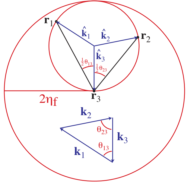
FIG. 12. Relationship between bispectrum triangle shapes and resonances in the three-point real space correlation function. As d \rightarrow 0 each set of self-similar bispectrum triangles determined by (\mathbf{k}_1, \mathbf{k}_2, \mathbf{k}_3)s , where s is some scale factor, causes a resonance at (\mathbf{r}_1, \mathbf{r}_2, \mathbf{r}_3) and its mirror image. As the overall size of the triangle s \rightarrow \infty this resonance becomes sharper and sharper in real space but remain associated with separations \mathcal{O}(\eta_f) . Flat triangles are responsible for the largest scale resonance for \mathbf{r}_1 - \mathbf{r}_3 = \mathbf{r}_2 - \mathbf{r}_3 = 2\eta_f .
