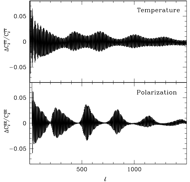
FIG. 8. Fractional angular power spectrum differences between the maximum likelihood sharp-step model ( A_C = 0.11, \eta_f = 8.163 Gpc) and pure power law model ( A_C = 0 ). The WMAP data prefer a few percent oscillation in the temperature power spectrum (top panel) around the first acoustic peak by 2\Delta \ln L = 11.6 . This model predicts matching E -polarization power spectrum oscillations (bottom panel) modulated by an orthogonal acoustic phase.
