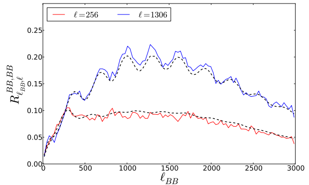
FIG. 5. Rows of the correlation matrix R , as in Fig. 4, between BB - BB bandpowers computed using either Monte Carlo simulations (solid lines) or our analytic model (dashed lines).
