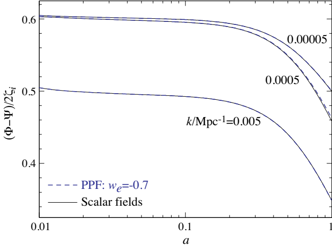
FIG. 1: PPF vs scalar field calculation of the evolution of the potential responsible for gravitational redshifts and lensing (\Phi - \Psi)/2 for a w_e = -0.7 model (flat, with \Omega_m = 0.31 and h = 0.64 ). Curves are normalized to the initial curvature \zeta_i .
