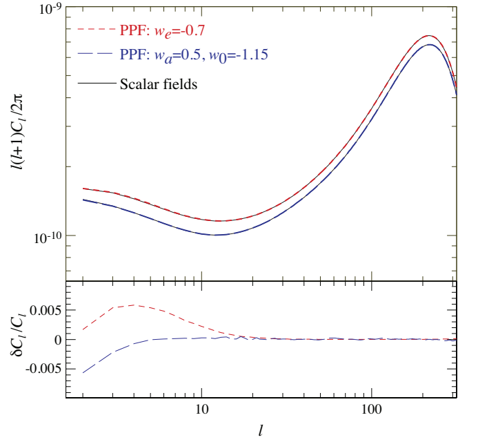
FIG. 2: PPF vs scalar field calculation of the CMB anisotropy power spectrum for the w_e = -0.7 model of Fig. 1 and a two-field crossing model that approximates w_0 = -1.15 and w_a = 0.5 (flat, with \Omega_m = 0.26 and h = 0.74 ).
