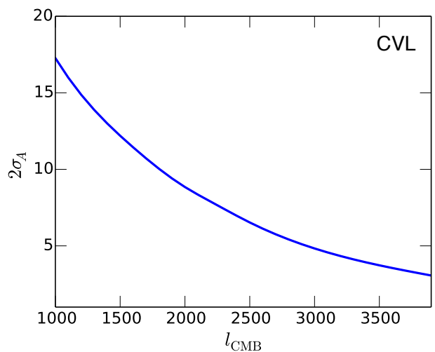
FIG. 5. 2\sigma detection threshold for the CVL case as a function of the maximum CMB multipole l_{\text{CMB}} used in reconstruction. Other parameters are set to the fiducial choices of Sec. IV A.
