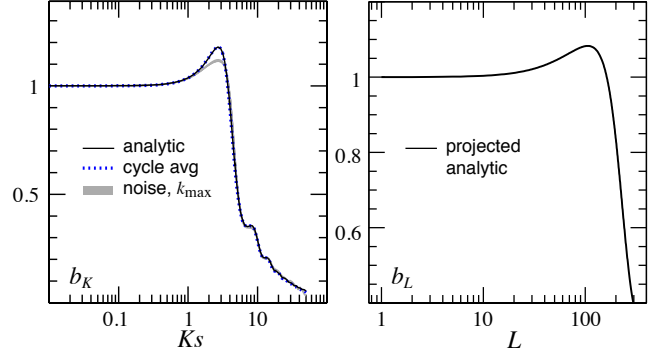
FIG. 7. Reconstruction bias in K (left) and in L (right) space. Left: analytic expression of Eq. (A19) is in excellent agreement with the evaluation of Eq. (A17) using the same cycle averaged replacement assumption \tilde{P}_{TT}(k) \rightarrow \langle \tilde{P}_{TT}(k) \rangle_x . Gray range shows the full calculation for a wide family of Poisson noise power spectra and k_{\text{max}} . Right: projected bias using the analytic expression from Eq. (A27) with \theta_* = 0.01 showing that L < 100 is nearly unbiased.
