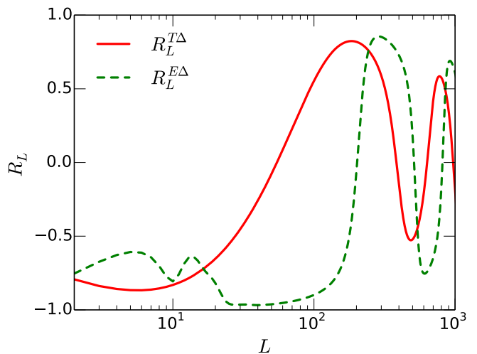
FIG. 1. Correlation coefficients R_L^{T\Delta} and R_L^{E\Delta} between the CIP and the CMB temperature and polarization fields respectively as a function of multipole L for A > 0 . The sign of the correlation oscillates due to acoustic oscillations in temperature and polarization whereas the level of correlation depends on the difference in projection effects between the fields.
