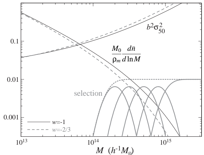
FIG. 4: Simulations predict the sample variance of counts, shown for a typical volume ( R = 50h^{-1} Mpc, upper curves), and the shape of the mass function (lower curves) as a function of mass. Self-calibration is assisted by binning the selection, multiplied here by 0.01 for clarity and shown here with \sigma_{\ln M} = 0.25 , into 5 bins of \Delta \log_{10} M^{\text{obs}} = 0.2 (solid lines) as opposed to a single threshold binning of M^{\text{obs}} \geq 10^{14.2} h^{-1} M_\odot (dotted line). With only threshold binning, joint changes to the cosmology, mass bias, and scatter are degenerate with the dark energy equation of state w (long dashed lines).
