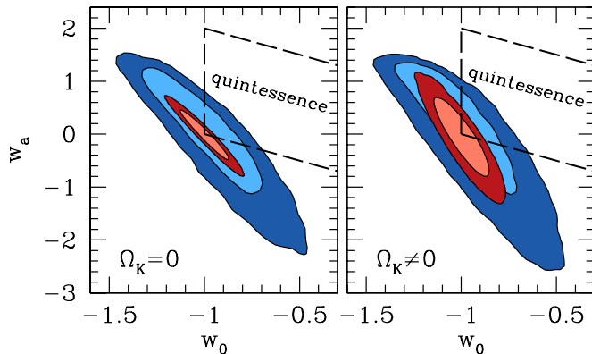
FIG. 3: Constraints on w_0 and w_a , assuming a flat universe (left panel) or marginalizing over spatial curvature (right panel). 68% CL (light shading) and 95% CL (dark shading) regions are shown for both current Union+WMAP constraints (outer contours, blue shading) and SNAP+Planck forecasts (inner contours, red shading). Dashed lines mark the boundary of the quintessence prior, -1 \leq w(z) \leq 1 .
