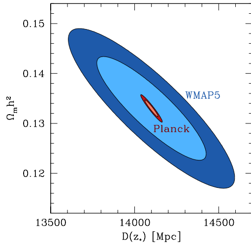
FIG. 2: Approximate constraints on D(z_*) and \Omega_m h^2 from WMAP 5-year data (outer contours, blue shading) and forecasts for Planck (inner contours, red shading), showing 68% CL (light shading) and 95% CL (dark shading) contours.
