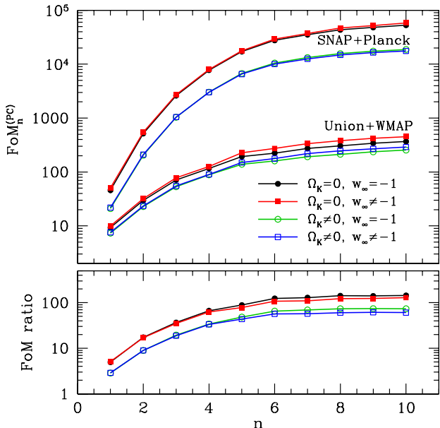
FIG. 6: Top panel: PC figures of merit \text{FoM}_n^{(\text{PC})} with forecasted uncertainties for SNAP+Planck and with measured uncertainties for Union+WMAP, normalized as in Eq. (10) to account for the quintessence prior. Bottom panel: Ratios of \text{FoM}_n^{(\text{PC})} forecasts to current values. In both panels, point types indicate different quintessence model classes: flat (solid points) or non-flat (open points), either with (squares) or without (circles) early dark energy.
