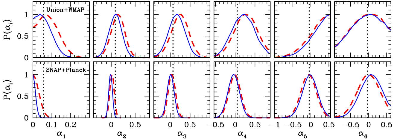
FIG. 5: Marginalized 1D posterior distributions for the first 6 PCs of flat (solid blue curves) and nonflat (dashed red curves) quintessence models without early dark energy. Marginalizing over the early dark energy parameter w_\infty has little effect on the distributions. Top row: current Union+WMAP data; bottom row: forecasts for SNAP+Planck assuming a realization of the data with \alpha_i = 0 . Plot boundaries that cut off the distributions at nonzero probability correspond to the top hat priors on \alpha_i for quintessence models. Higher variance PCs are mainly limited by the quintessence priors for both current constraints and forecasts (see Table II). Vertical dotted lines show the predictions of an example quintessence model from Eq. (12) (see Fig. 4).
