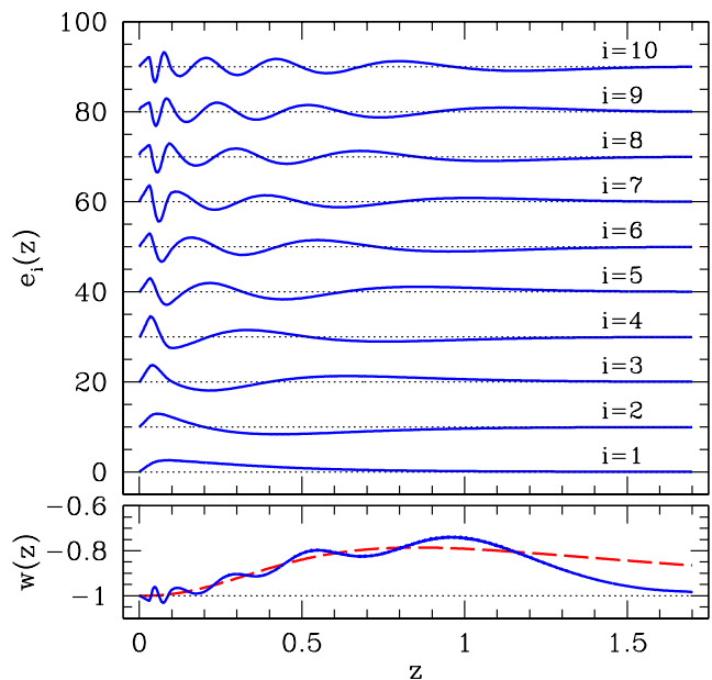
FIG. 4: Top panel: The first 10 PCs of w(z) (increasing variance from bottom to top), with 500 redshift bins between z = 0 and z_{\max} = 1.7 . The PCs are offset vertically from each other for clarity. Bottom panel: an example of w(z) for a quintessence model (red dashed curve; see Eq. (12)) and its representation using the first 10 PCs in Eq. (7) (blue solid curve). Dotted lines show the w = -1 zero point for each component (top) and for the example model (bottom).
