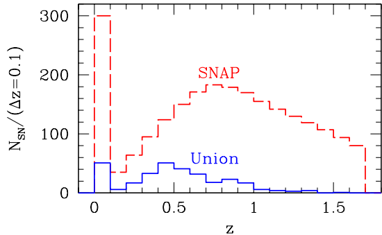
FIG. 1: Redshift distributions of Type Ia supernovae in the Union compilation (solid blue) and assumed for SNAP (dashed red), including the anticipated low-redshift sample from other surveys at z < 0.1 .
