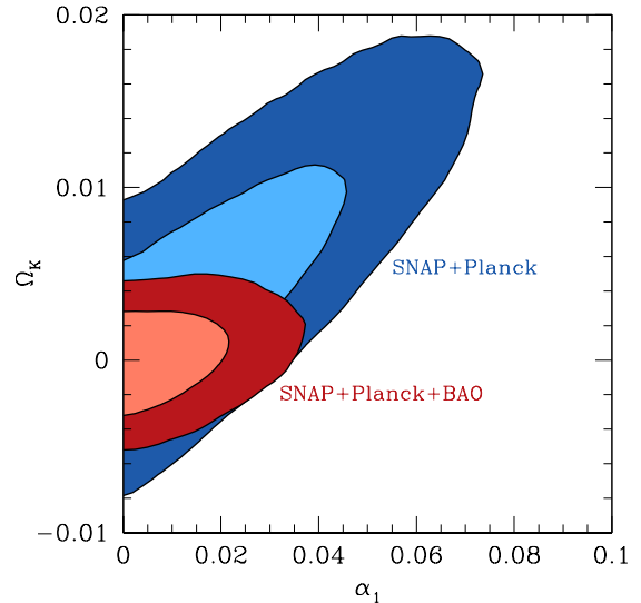
FIG. 7: Forecasts for \Omega_K and the amplitude of the first PC, \alpha_1 , showing 68% CL (light shading) and 95% CL (dark shading) regions. The large contours (blue shading) include only SNAP and Planck data as well as the additional priors from Sec. II C. The small contours (red shading) add to these data a 1% measurement of \langle D_V \rangle averaged over the redshift bin 0.8 < z < 1.2 as might be obtained from a future BAO experiment, reducing the degeneracy between curvature and dark energy.
