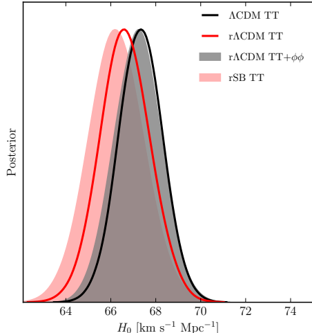
FIG. 6. H_0 and inflationary parameters. In phase \ell > 1000 residuals in Fig. 3 drive H_0 lower than the \Lambda CDM TT model (black) but require running parameters (red curve, rACDM; red shaded, rSB) in order to produce a global fit. These fits also predict more gravitational lensing and are not favored by lensing reconstruction data (gray shaded, rACDM TT+ \phi\phi ).
