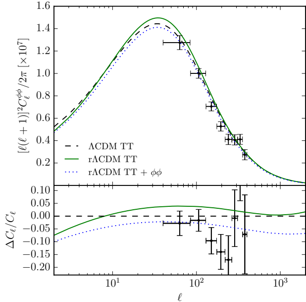
FIG. 7. Lensing power spectrum in the \Lambda CDM TT model vs. running models rACDM TT and rACDM TT+ \phi\phi . Lowering H_0 in the rACDM model simultaneously raises lensing and is not favored once the lensing reconstruction data (points) are taken into account.
