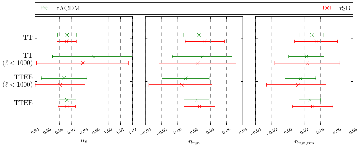
FIG. 11. Constraints on inflationary parameters – tilt, its running, and the running of the running from Eq. 2 – for the 4 combinations of datasets in Tab. I.
