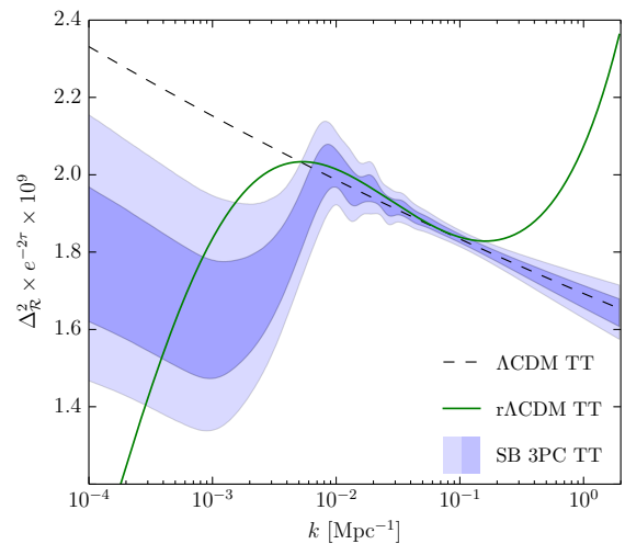
FIG. 16. Functional reconstruction of inflationary power spectrum ( \Delta_{\mathcal{R}}^2 : 68%, 95% CL) from the first 3 principal components in the SB TT (shaded) analysis compared with the best fit running model r\Lambda\text{CDM TT} .
