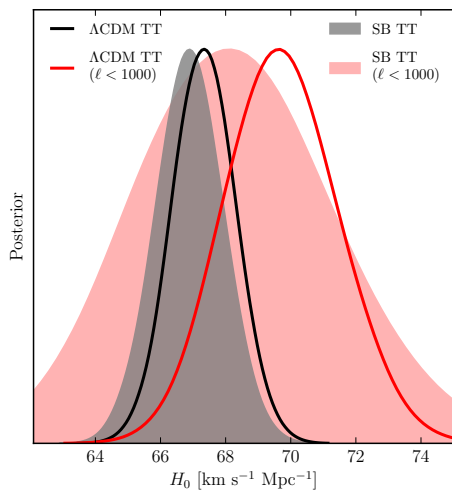
FIG. 4. H_0 from the TT full vs ( \ell < 1000 ) datasets. Low- \ell residuals in Fig. 3 drive H_0 higher in the \Lambda CDM TT ( \ell < 1000 ) analysis (red vs black curves). In the SB model, these residuals are fit by inflationary rather than cosmological parameter changes, so low values of H_0 that are favored in the full analysis (gray shaded) are also compatible in the ( \ell < 1000 , red shaded) analysis.
