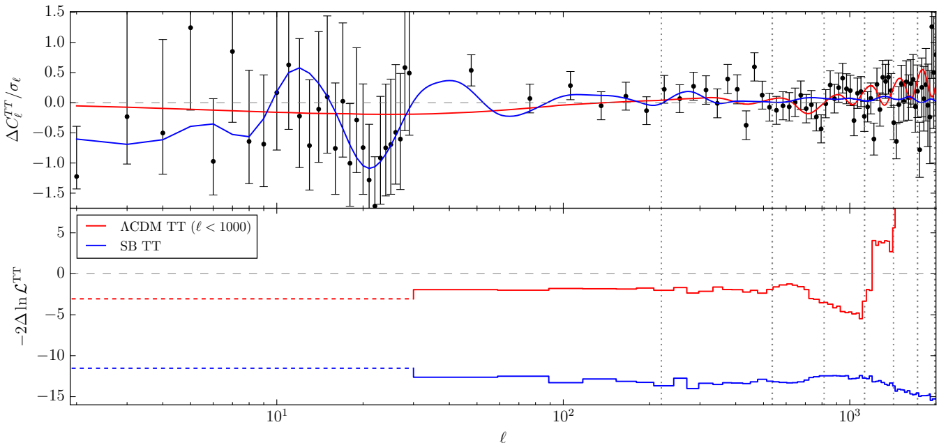
FIG. 3. Top panel: residuals in the TT data (points) and models relative to the best fit \Lambda CDM TT model of Tab. III (dashed line). Bottom panel: change in the likelihood 2\Delta \ln \mathcal{L}^{\text{TT}} of models relative to \Lambda CDM TT starting from the lowest bin at 2 \leq \ell < 30 (dotted lines) and adding each individual data point thereafter. The \Lambda CDM TT ( \ell < 1000 ) model (red line) fits the residuals at low \ell \lesssim 40 and \ell \sim 700 - 1000 better due to changes in H_0 and other parameters, but it is a poor fit to the in-phase residuals at \ell > 1000 . Conversely, the inflationary feature SB model (blue) fits the low- \ell residuals yielding a large 2\Delta \ln \mathcal{L}^{\text{TT}} \sim 12 improvement at low \ell , but only small changes at high \ell . Note that the \Lambda CDM TT ( \ell < 1000 ) model has the same foreground parameters as the \Lambda CDM TT model, and the data points assume TT foregrounds are fixed to the best fit \Lambda CDM TT values in Ref. [9].
