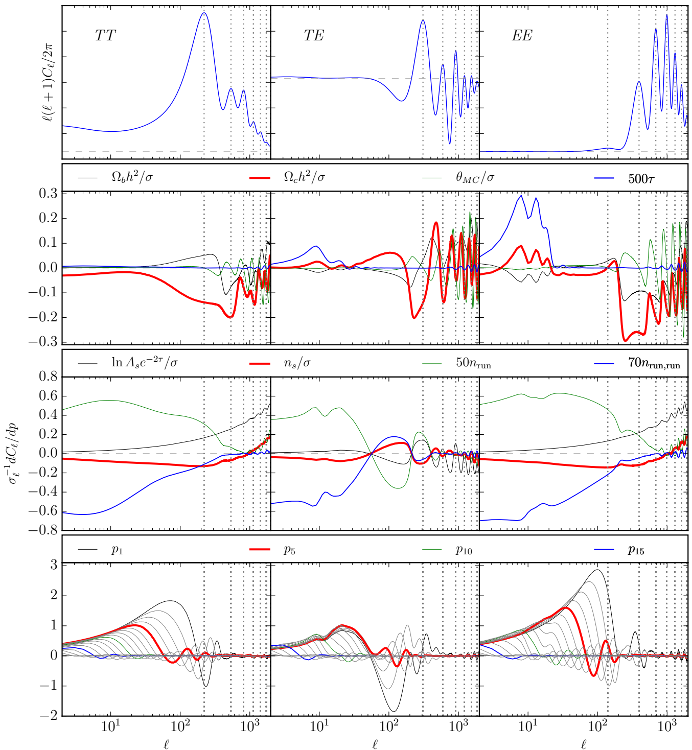
FIG. 1. Response of the TT, TE, EE power spectra to various parameters around the \Lambda CDM TT model of Tab. III. Derivatives are scaled by \sigma_\ell , the cosmic variance error per \ell of the model, and parameters are scaled by either their Planck 2015 \Lambda CDM TT error \sigma or by a fixed number for visibility. Vertical dotted lines are drawn at the acoustic peak locations and horizontal dashed lines at zero levels.
