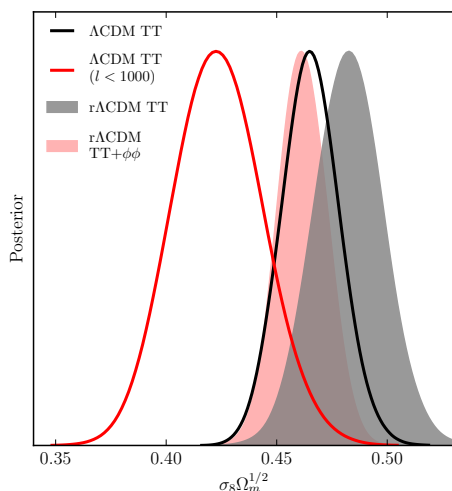
FIG. 10. Amplitude of structure \sigma_8 \Omega_m^{1/2} . Shifts in \Omega_c h^2 from \Lambda CDM TT ( \ell < 1000 ; red curve) to the full range (black curve) drive \sigma_8 \Omega_m^{1/2} higher. Fitting the in-phase high- \ell residuals with the enhanced freedom of the r \Lambda CDM model drives it even higher (gray shaded), but in a manner inconsistent with the lensing reconstruction data (red shaded).
