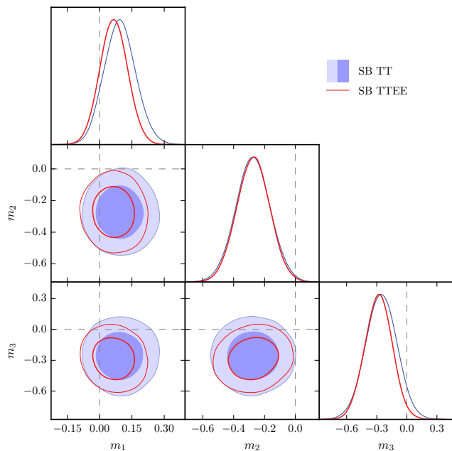
FIG. 14. First 3 principal components of the SB TT p_i covariance matrix in the TT (thin blue) and TTEE (thick red) analysis (68%, 95% CL). Both m_2 and m_3 show non-zero deviations whose significance is slightly enhanced by the addition of polarization information.
