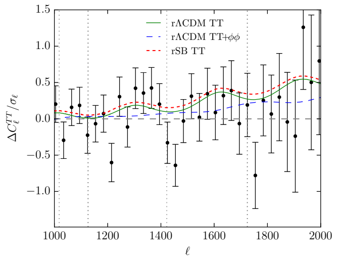
FIG. 5. TT residuals at \ell > 1000 relative to the best fit \Lambda CDM TT model of Tab. III (dashed line). With the running parameters, rACDM and rSB seek to fit the oscillatory residuals and make the peaks smoother. Adding the lens reconstruction data \phi\phi largely removes this preference.
