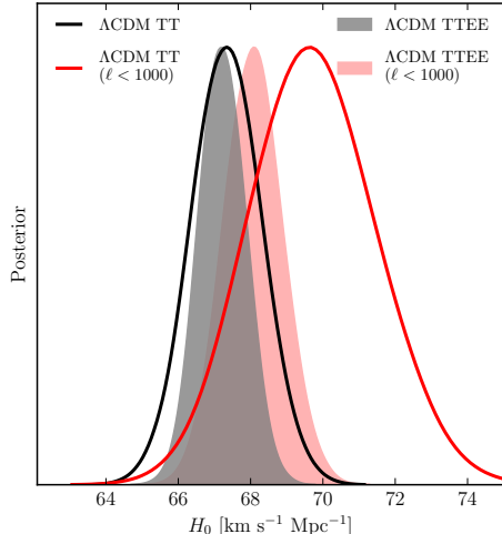
FIG. 8. H_0 and polarization data. TE residuals shown in Fig. 9, especially near \ell \sim 200 , drive H_0 lower, even in the \ell < 1000 datasets (red curves to red shaded), whereas the full data range provide values consistent with \Lambda CDM TT, with smaller errors.
