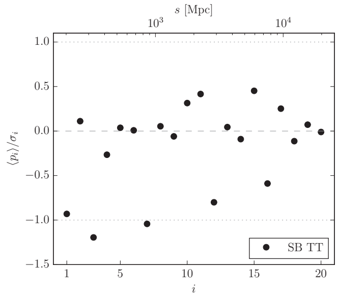
FIG. 13. SB parameters of the SB TT analysis in units of their errors. No single SB parameter p_i is significantly detected due to covariances hidden in the marginalized errors.
