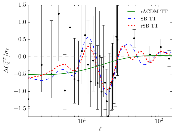
FIG. 12. Low- \ell TT residuals (points) and models relative to the best fit \Lambda CDM TT model of Tab. III (black dashed). While the running model rACDM TT (green solid) can suppress power, the SB TT model (blue dashed) accommodates the sharp dip favored by the data. Allowing both running and SB in the rSB TT model (red dotted) leads to a similar fit as SB TT.
