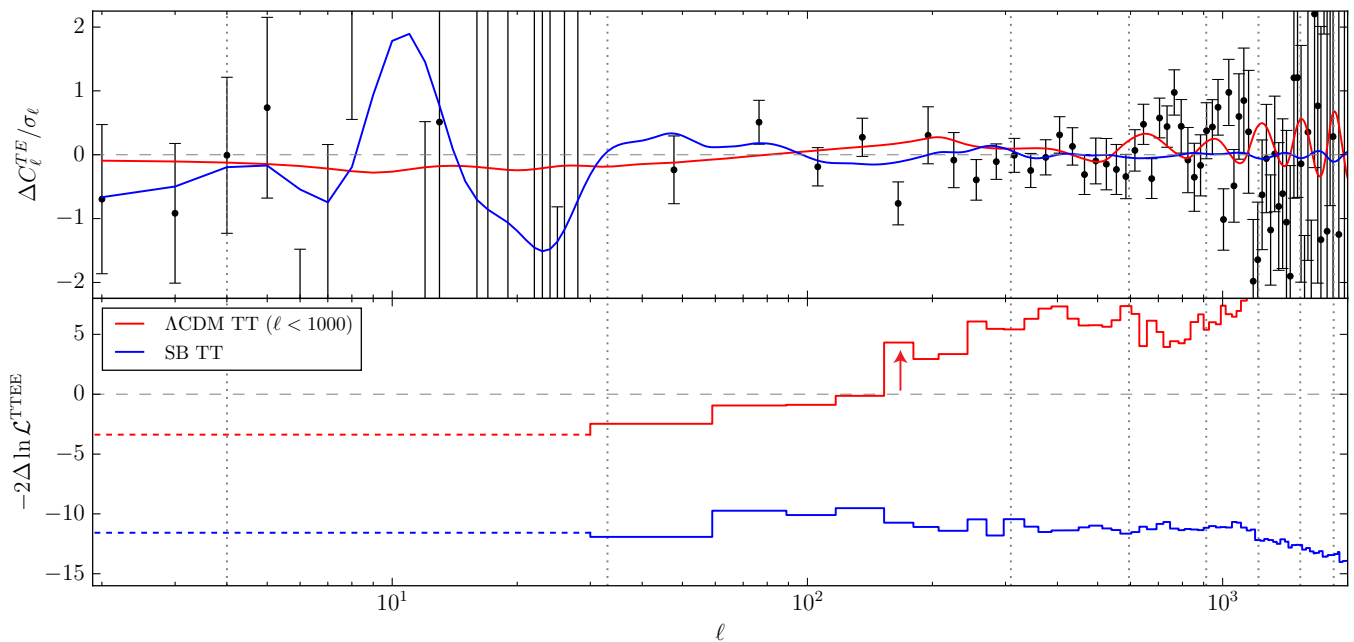
FIG. 9. Top panel: residuals in the TE data (points) and the same models as in Fig. 3 relative to the best fit \Lambda CDM TT model of Tab. III (dashed line). Bottom panel: -2\Delta \ln \mathcal{L}^{\text{TTEE}} of models relative to \Lambda CDM TT in the same form as Fig. 3. Cosmological parameters are fixed to their TT best fit values and the TT ( \ell < 1000 ) model also has the same foreground parameters as the TT model including polarized foregrounds. The \Lambda CDM TT ( \ell < 1000 ) model becomes a worse fit to the TTEE dataset when passing the outlier point at \ell \approx 165 (arrow), whereas the SB TT model slightly improves the fit.
