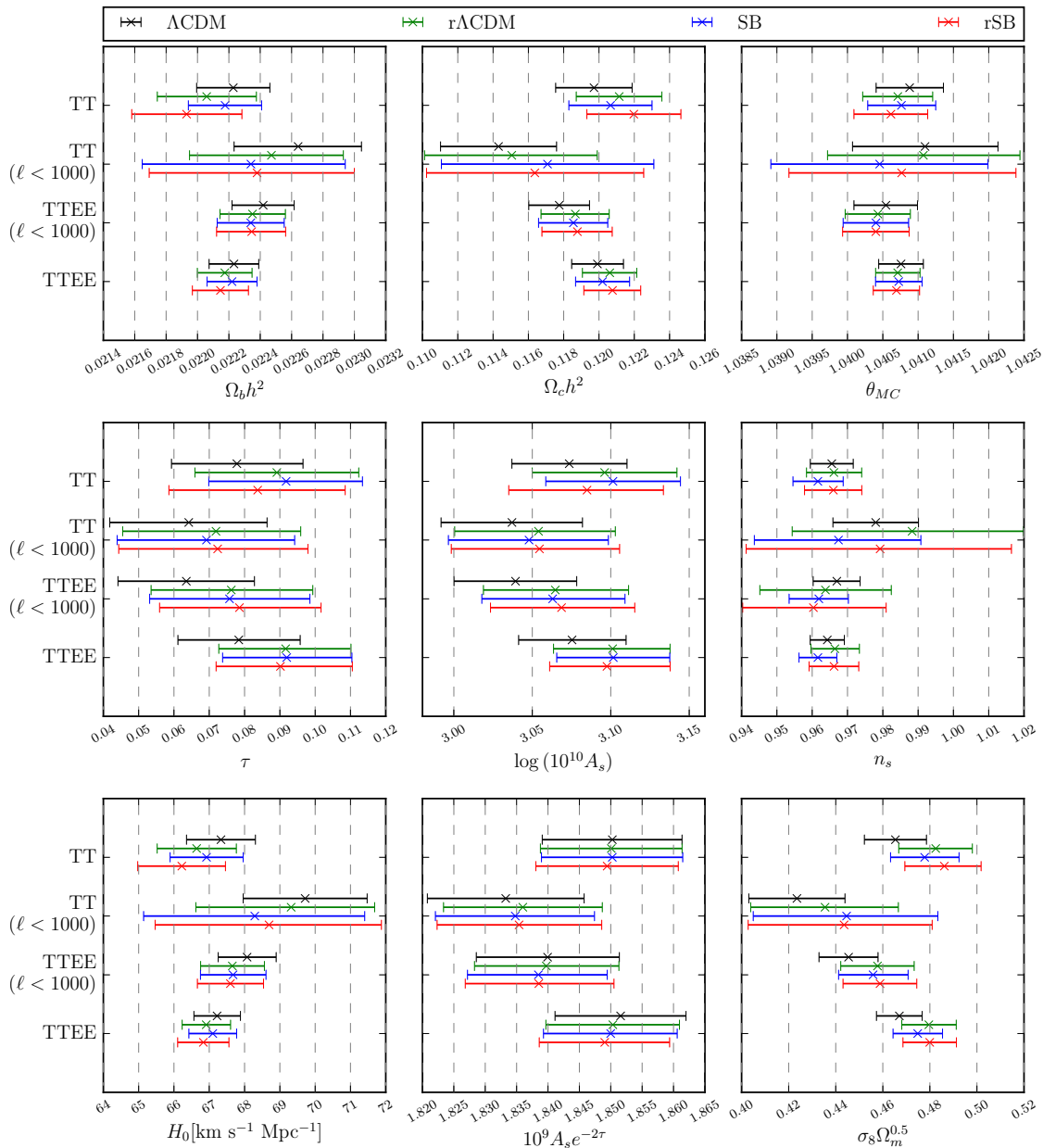
FIG. 2. Cosmological parameter constraints with the 4 combinations of datasets in Tab. I on the 4 models for the inflationary power spectrum in Tab. II.
