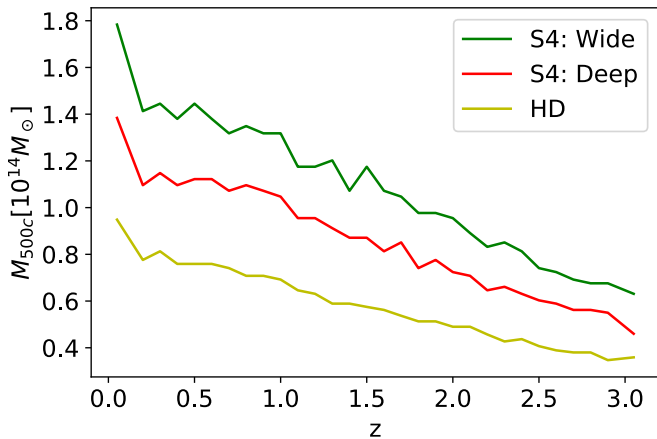
FIG. 2. The mass detection limit M_{\text{lim}} as a function of redshift from Ref. [30], linearly interpolated between their \Delta z = 0.1 bins.
