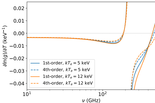
FIG. 5. The fractional response of the tSZ spectrum, with 1st-order and 4th-order relativistic corrections, to the temperature of the cluster. Here we take \mu = 0 for a cluster with k_B T_e = 5 keV and another with k_B T_e = 12 keV.
