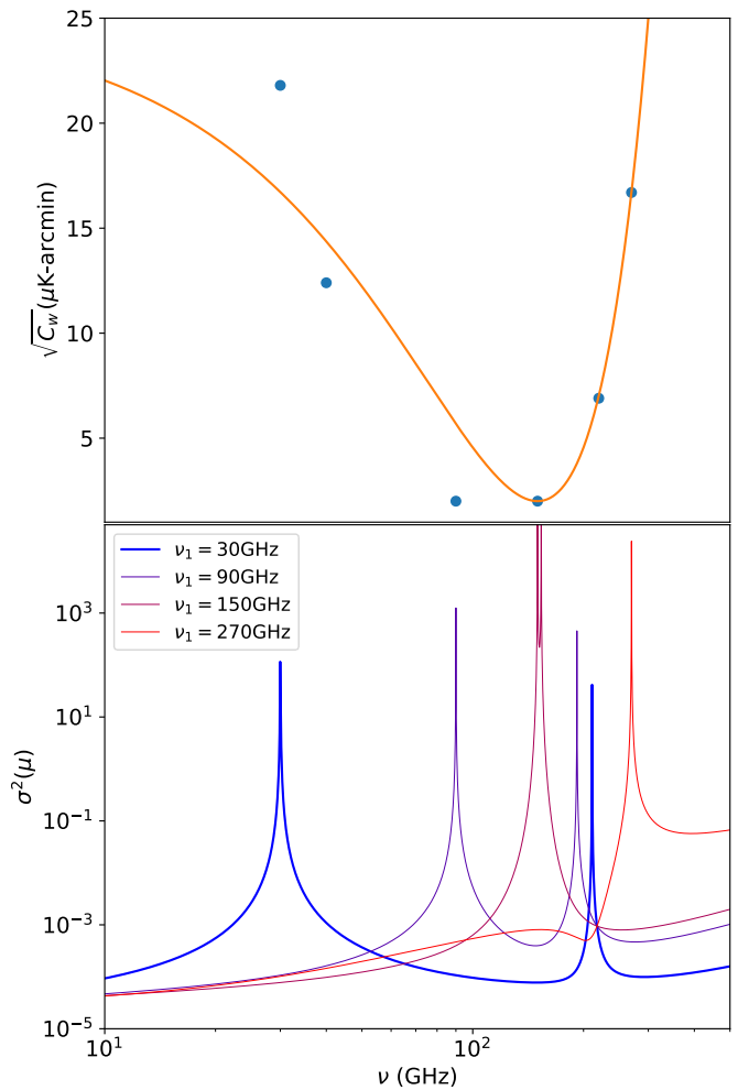
FIG. 4. Top: Frequency scaling relation for \sqrt{C_w} . Blue points correspond to the S4-Wide survey’s specifications. Bottom: \sigma^2(\mu) for different frequency pairs for a single cluster with y_c = 10^{-4} and \theta_c = 1 arcminute. We see that the constraints on \mu improve when the channels are separated from each other, rather than being closely spaced. In general, we see that as long as there is a separation, lower frequency channels provide more sensitivity to \mu in this baseline case of white detector noise only, in accordance with Fig. 1.
