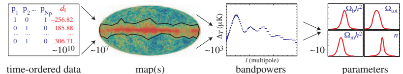
Figure 5: Data pipeline and radical compression. Map are constructed for each frequency channel from the data timestreams, combined and cleaned of foreground contamination by spatial (represented here by excising the galaxy) and frequency information. Bandpowers are extracted from the maps and cosmological parameters from the bandpowers. Each step involves a substantial reduction in the number of parameters needed to describe the data, from potentially 10^{10} \rightarrow 10 for the Planck satellite.
