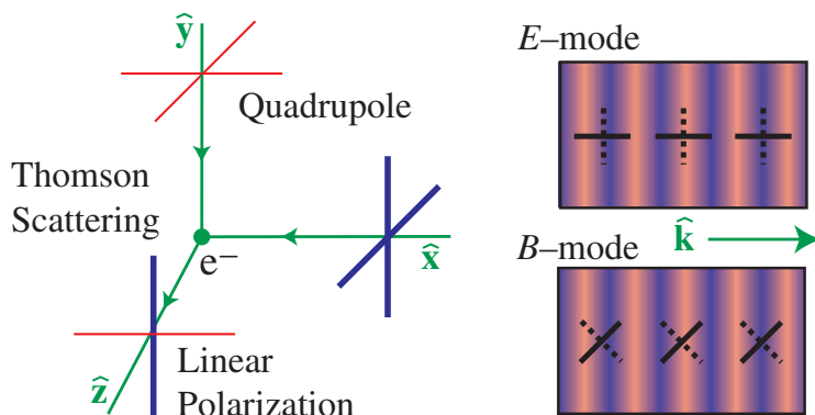
Plate 2: Polarization generation and classification. Left: Thomson scattering of quadrupole temperature anisotropies (depicted here in the \hat{x} - \hat{y} plane) generates linear polarization. Right: Polarization in the \hat{x} - \hat{y} plane along the outgoing \hat{z} axis. The component of the polarization that is parallel or perpendicular to the wavevector \mathbf{k} is called the E -mode and the one at 45^\circ angles is called the B -mode.
