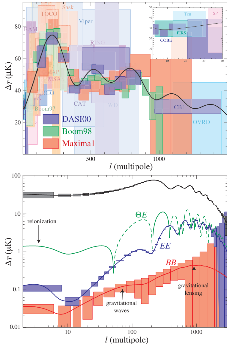
Plate 1: Top: temperature anisotropy data with boxes representing 1\text{-}\sigma errors and approximate \ell -bandwidth. Bottom: temperature and polarization spectra for \Omega_{\text{tot}} = 1 , \Omega_\Lambda = 2/3 , \Omega_b h^2 = 0.02 , \Omega_m h^2 = 0.16 , n = 1 , z_{\text{ri}} = 7 , E_i = 2.2 \times 10^{16} GeV. Dashed lines represent negative cross correlation and boxes represent the statistical errors of the Planck satellite.
