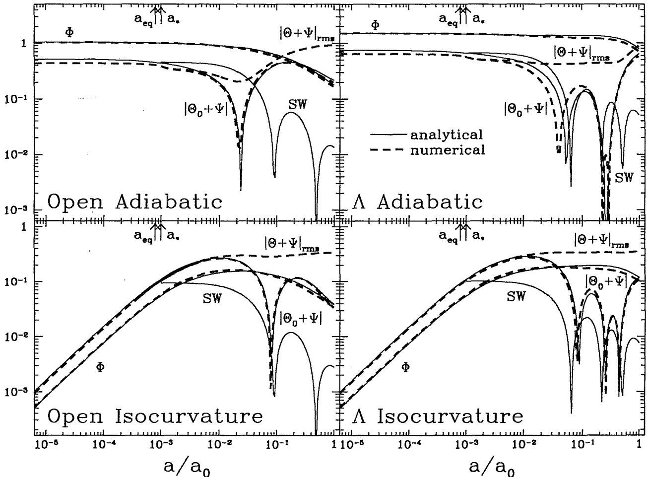
FIG. 2. The evolution of total Sachs-Wolfe effect ( \Omega_0 = 0.1 , h = 0.5 , k = 4 \times 10^{-4} \text{ Mpc}^{-1} standard recombination). In the adiabatic case, temperature fluctuations are enhanced in gravitational wells such that \Theta and \Psi partially cancel, yielding \Theta_0 + \Psi = \frac{1}{3}\Psi in the matter-dominated epoch. For the isocurvature case, the ISW effect creates a net total of \Theta_0 + \Psi = 2\Psi reflecting the anticorrelated nature of radiation and total density fluctuations. After last scattering at a_* , this SW contribution [analytic only, Eq. (31)] collisionlessly damps from the monopole. The rms temperature fluctuations [numerical only, Eq. (10)] acquire contributions after a_* from the ISW effect due to the radiation (early) and curvature or \Lambda (late) contributions. These contributions are relatively more important for, Eq. (10) adiabatic models due to the partial cancellation of \Theta_0 and \Psi at last scattering. Since \Lambda domination can only have occurred comparatively recently, the late ISW effect is also less important in a \Lambda compared to an open universe.
