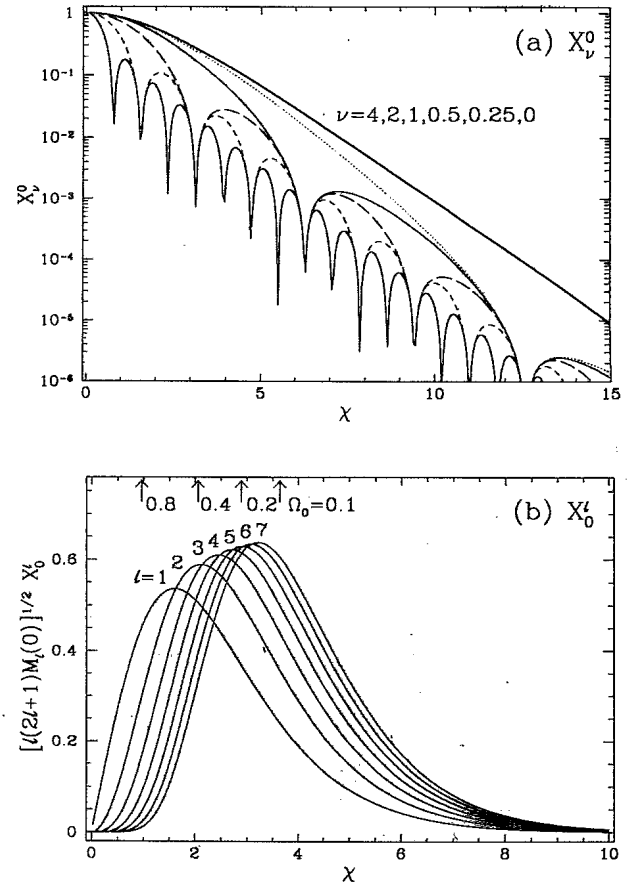
FIG. 23. Radial eigenfunctions of an open universe X_\nu^l(\chi) . (a) The isotropic l = 0 function for several values of the wave number \nu = \tilde{k}/\sqrt{-K} . The zero crossing moves out to arbitrarily large scales as \nu \rightarrow 0 , reflecting completeness. However, even as this “effective wavelength” becomes infinite, the function retains prominent structure only near the curvature scale \chi = 1 . A random superposition of these low \nu modes cannot produce more than exponentially decaying structure larger than the curvature scale. (b) Low-order multipoles in the asymptotic limit \nu \rightarrow 0 . If most power lies on the curvature scale, the l mode corresponding to the angle that the curvature radius subtends will dominate the anisotropy. The normalization is appropriate for comparing contributions to the anisotropy l(2l + 1)C_l/4\pi . Also shown is the location of the horizon \chi = \eta_0\sqrt{-K} for several values of \Omega_0 . If contributions to the anisotropy come from a sufficiently early epoch, the dominant l mode will peak at this value.
