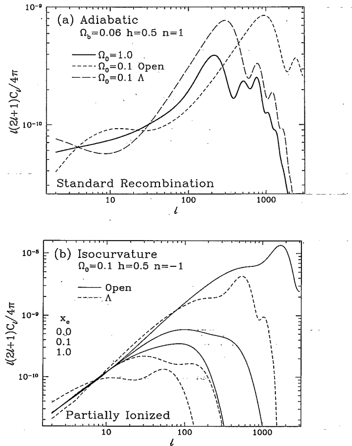
FIG. 21. Intermediate- to small-scale anisotropies. (a) Adiabatic models. Projection of the sound horizon at last scattering onto the sky today determines the angular scale of the “Doppler peaks” (cf. Fig. 11). The sound horizon is the same physical scale for open and \Lambda models with fixed \Omega_0 but geodesic deviation makes it correspond to a smaller angle in the open case. Compared with the flat case, the \Lambda model has a somewhat smaller angular scale due to the imperfect cancellation between the increase in the age of the Universe today and at last scattering. (b) Isocurvature models. Anisotropies in the standard recombination scenario ( x_e \simeq 0 ) produce far too large fluctuations on arcminute scales due to the steeply rising spectrum. Reionized models have their adiabatic fluctuations damped out by photon diffusion and a cancellation suppressed Doppler effect. Notice that large-angle anisotropies are immune to ionization history effects for the open case but not for the \Lambda case. This and the difference in the damping scale are mostly due to the projection effect.
