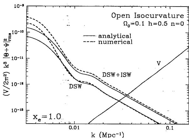
FIG. 22. Isocurvature temperature power spectrum. In this fully ionized x_e = 1 , low \Omega_0 = 0.1 , h = 0.5 model, the ISW effect makes a contribution equal to and with the same scale dependence as the cancelled Doppler (plus SW) term (DSW). The second-order Vishniac term ( V ) dominates at small scales. The analytic approximation (solid) fails at large scales where cancellation arguments are not applicable.
