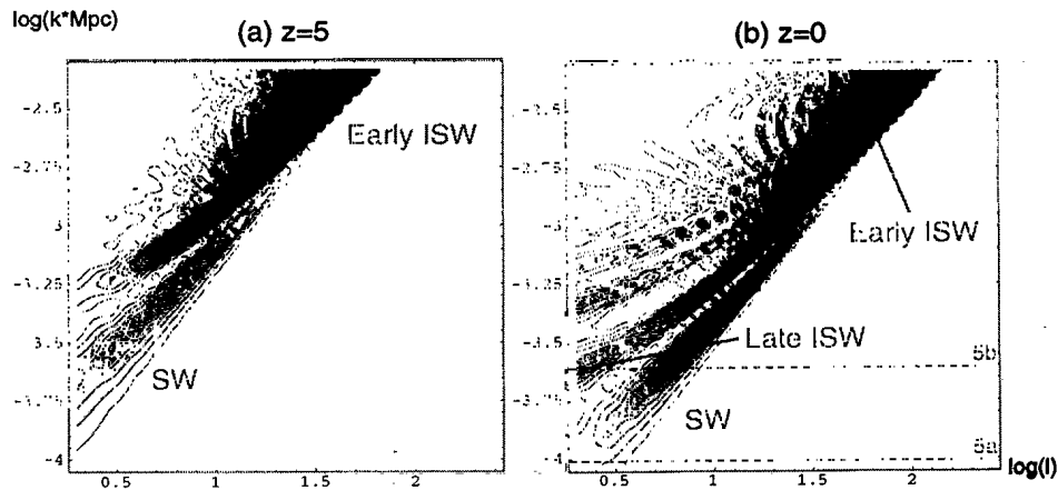
FIG. 4. \Lambda adiabatic photon spectrum ( \Omega_0 = 0.1 , h = 0.5 , standard recombination). Unlike the \Omega_0 = 1 case, this scenario has significant contributions from after last scattering through the early and late ISW effect. (a) The early ISW effect arises if horizon crossing is near radiation domination, and projects onto a second ridge which is more prominent than the SW ridge at intermediate but not large angles. (b) After \Lambda domination, the late ISW contributions come free streaming in from the monopole yielding a boost in the low-order multipoles for a small range in k , due to cancellation with SW contributions at the largest scales and crest-trough cancellation at smaller scales. Scales depicted in Figs. 5(a) and 5(b) are marked here by dashed lines. The logarithm is to base 10.
