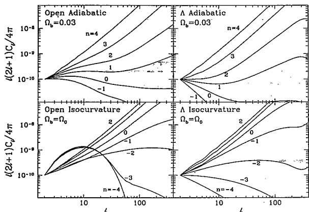
FIG. 19. Large-angle anisotropy dependence on the initial power spectrum |C_l|^2 \propto \tilde{k}^n or |C_A|^2 \propto \tilde{k}^n for isocurvature and adiabatic scenarios, respectively. ( \Omega_0 = 0.1 , h = 0.5 , standard recombination.) Notice that for red spectra, geometric and/or cosmological constant effects play a role in determining the anisotropy whereas for very blue spectra, l^2 C_l \propto l^2 for all models. Isocurvature models with n \simeq -1 to fit large-scale structure will thus not be extremely sensitive to open or \Lambda dominated universe effects. The normalization here is arbitrarily matched at the quadrupole.
