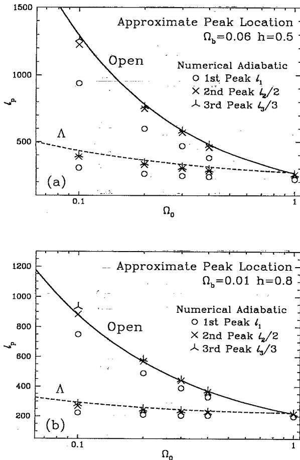
FIG. 11. Angular scale of the "Doppler peaks" (standard recombination). The physical scale of the peaks is simply related to the sound horizon at last scattering. Peaks in the anisotropy today will correspond to multiples of the angle that this scale subtends on the sky l_p = \pi r_\theta / r_s(\eta_*) , as discussed in the text. Varying \Lambda or h increases both the sound horizon at \eta_* and the present horizon \eta_0 leaving little effect. For open models, a given scale will correspond to a smaller angle by geodesic deviation. This simple analytic estimate (lines) for the peak location is valid for pure acoustic contributions and underestimates the scale of the first peak in low \Omega_0 h^2 models due to neglect of the early ISW effect.
