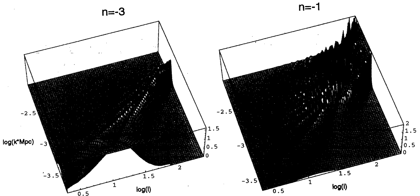
FIG. 20. The full open isocurvature photon power spectrum for |C_l|^2 \propto \bar{k}^n . (a) Curvature scale weighted n = -3 . The lack of a Poisson cutoff in the isocurvature potential makes the nature of the open universe eigenfunctions apparent. The projection ridge crosses minimum eigenvalue k = \sqrt{-K} (front edge) at roughly l \sim 10 , corresponding to the fact that the lowest eigenfunction still has structure only around the curvature scale. This leads to the cutoff to low multipoles depicted in Fig. 19. (b) Small-scale weighted n = -1 . The main projection ridge does not dominate the anisotropy at the low-order multipoles. Power from smaller physical scales (high k ) bleeds in to boost the anisotropy. Thus anisotropies do not rise as rapidly with l as predicted from the one-to-one conversion of k onto l . For this model n_{\text{eff}} \simeq 2 at large angles. The logarithm is to base 10.
