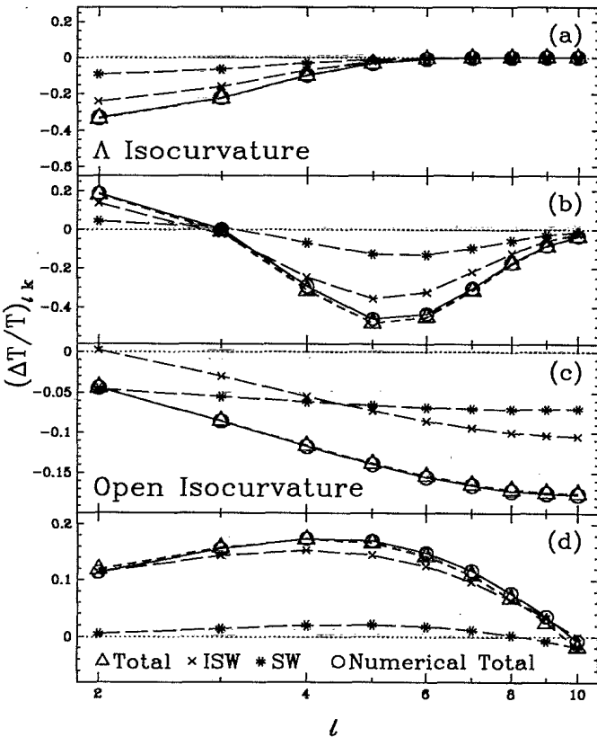
FIG. 8. Analytic separation of isocurvature large angle anisotropies ( \Omega_0 = 0.1 , h = 0.5 , standard recombination, arbitrary normalization). Scales are chosen to match the features in Fig. 7. In general, isocurvature models have strong early ISW contributions which mimic and coherently boost the SW effect. \Lambda models: (a) Notice that the shape of the SW and ISW effects are identical at large scales. (b) Even at the late ISW peak, the early ISW contributions are so strong that the late contributions are never apparent, unlike the adiabatic model. Open models: (c) As with \Lambda models, radiation epoch contributions are significant making the SW and ISW contributions similar for large scales. (d) Near the peak of the curvature ISW contribution however, the relative contributions are similar to the adiabatic case.
