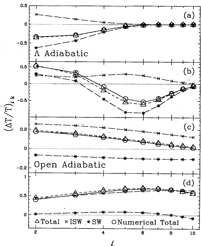
FIG. 5. Analytic separation of adiabatic large-angle anisotropies ( \Omega_0 = 0.1 , h = 0.5 , standard recombination, arbitrary normalization). Scales are chosen to match the features in Figs. 4 and 6. \Lambda models: (a) At the largest scales, e.g., here k = 10^{-4} \text{ Mpc}^{-1} , the SW effect increasingly dominates over the late ISW effect due to projection. However, since the potential decays, the late ISW effect partially cancels the SW effect if the mode is superhorizon sized at \Lambda domination. (b) Intermediate-scale peaks in Fig. 4 are due to the late ISW boost of the higher SW free-streaming ridges. Open models: (c) The maximum scale corresponds to the curvature radius k = \sqrt{-K} . For this scale, the SW effect projects broadly in l peaking near l \sim 10 . For the late ISW effect, this scale projects onto the monopole and dipole near curvature domination thus leaving the ISW contributions to decrease smoothly with l . (d) At smaller scales, corresponding to the large ridge in Fig. 6, the late ISW effect projects onto l \simeq 2-10 and completely dominates leading to a rising spectrum of anisotropies.
