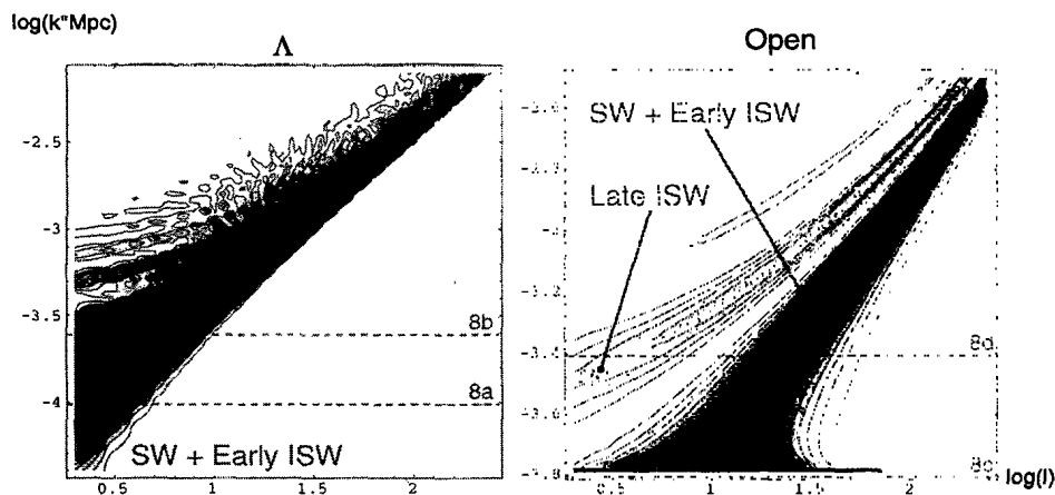
FIG. 7. \Lambda and open isocurvature photon spectrum ( \Omega_0 = 0.1 , h = 0.5 , standard recombination). Unlike their adiabatic counterparts, the potential grows in the radiation domination era only to turn over and decay in the curvature and \Lambda dominated era. The early ISW contribution will thus smoothly match onto the SW contribution. This has the effect of merging the SW and ISW ridges to make a wide feature that contributes broadly in l . For \Lambda models, the early ISW effect completely dominates over the late ISW effect. Scales depicted in Fig. 8 are marked here by dashed lines. The logarithm is to base 10.
