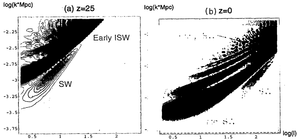
FIG. 6. Open adiabatic photon spectrum ( \Omega_0 = 0.1 , h = 0.5 , standard recombination). (a) Like the \Lambda case, the early ISW effect contributes significantly to intermediate angle anisotropies. (b) However, as already noted in Fig. 2, the late ISW effect appearing at the left is much more significant than the corresponding \Lambda effect. Thus on all angular scales, the total ISW contribution dominates the SW effect. Contours curve away from the curvature scale \log_{10}(k \text{ Mpc}) = -3.8 due to suppression of the potentials from the Poisson equation. Scales depicted in Figs. 5(c) and 5(d) are marked here with dashed lines. The logarithm is to base 10.
