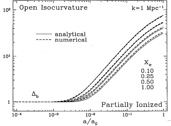
FIG. 13. Open isocurvature baryon evolution under partial ionization ( \Omega_0 = 0.2 , h = 0.5 ). The baryons are released to grow in pressureless linear theory after Compton drag becomes negligible. Since this epoch becomes earlier as the ionization fraction is decreased, present-day fluctuations will be larger for low x_e , if normalized to the ionization independent fluctuations at large scales. Unlike the CDM base, baryons have no potential wells into which they might fall after the drag epoch and the transfer function is extremely sensitive to the ionization history.
