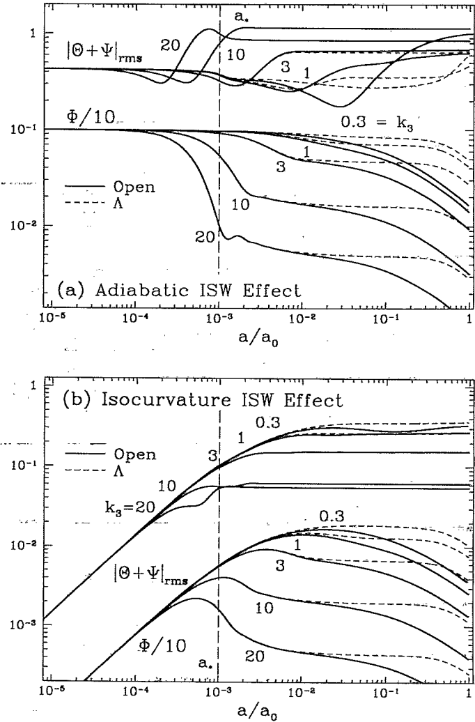
FIG. 12. The total ISW effect on |\theta + \Psi|_{\text{rms}} ( \Omega_0 = 0.1 , h = 0.5 , standard recombination, k = k_3 \times 10^{-3} \text{ Mpc}^{-1} ). (a) Adiabatic models ( \Omega_b = 0.06 ). The decay of the potential as the scale enters the horizon due to pressure growth suppression causes the early ISW effect which boosts scales approaching the first acoustic oscillation. The largest scales which enter after radiation domination are boosted by the late ISW effects due to the rapid expansion in open and \Lambda models, leaving a deficit at intermediate scales. (b) Isocurvature models ( \Omega_0 = \Omega_0 ). Scales which enter early during radiation domination do not grow as much due to the suppression in the potential. This enhances the large scales with respect to the small. Notice that the second adiabatic oscillation ( k_3 = 20 ) can be comparable to the first since the turnover in \Phi occurs later. Only at the largest scales is the distinction between open and \Lambda models manifest in the rms temperature fluctuations.
