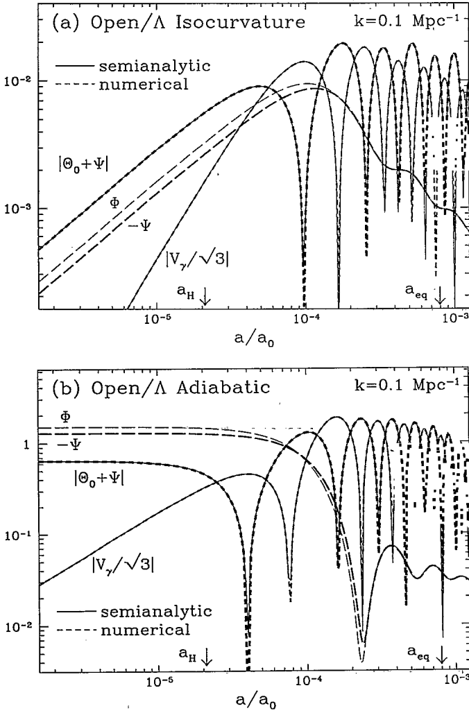
FIG. 9. The acoustic oscillations ( \Omega_0 = 0.2 , h = 0.5 , no recombination). The photon-baryon fluid acts like an oscillator in a potential well. The dipole, i.e., the photon velocity V_\gamma , is increasingly suppressed with respect to the monopole as (1+R)^{-1/2} , where the \sqrt{3} accounts for the three degrees of freedom in the dipole. Scales which reach an extrema in the monopole at last scattering will correspond to the so-called ‘‘Doppler peaks’’ in the anisotropy spectrum. Also displayed here is the semianalytic approximation described in the text, which is essentially exact. The small difference in the numerical amplitudes of \Phi and \Psi is due to the anisotropic stress of the neutrinos. Whereas the isocurvature case has \Omega_0 = \Omega_b , the adiabatic model has \Omega_b = 0.06 and a consequently smaller R .
