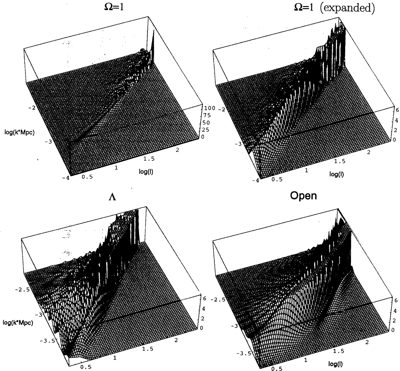
FIG. 18. The full adiabatic photon power spectrum. The logarithmic contributions to the anisotropy in l and k [see Eq. (9)] are plotted here. Whereas in the \Omega_0 = 1 case only the SW ridge and acoustic peaks are prominent ( top left and close up, top right ), the \Lambda and open cases show more complicated structure due to the ISW effect. Depending on the initial weightings, represented here as |C_A|^2 \propto \bar{k} , certain features may be emphasized over others. Notice the \Lambda late ISW effect at low l and intermediate k and the comparatively small open SW contribution at the foot of the ISW ridge. The logarithm is to base 10.
