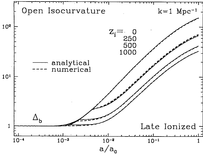
FIG. 14. Open isocurvature baryon evolution in late reionization scenarios ( \Omega_0 = 0.2 , h = 0.5 ). Here the Universe is suddenly reionized to x_e = 1 at redshift z_i after a transparent period 1000 > z > z_i . Perturbations are released from drag following recombination only to suffer its effects once again between the ionization and drag epochs z_i > z > z_d . Thus the final fluctuations will be larger for later reionization.
