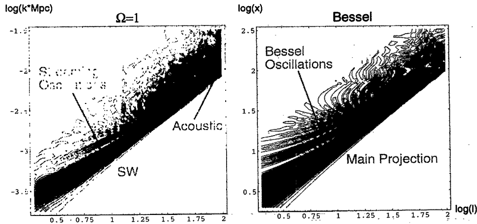
FIG. 3. \Omega_0 = 1 adiabatic full photon spectrum ( h = 0.5 , standard recombination, left panel). Shown here and in Figs. 4, 6, and 7 is the contribution to the anisotropy per logarithmic k and l interval (\Delta T/T)_{lk}^2 [Eq. (9)] with equally spaced contours up to a cutoff set to best display the features in question. The strong correlation between l and k merely reflects the projection of a scale on the last scattering surface to an angle on the sky. At \log_{10} l \gtrsim 2 , SW contributions fall off and are replaced by the acoustic peaks (saturated here). The detailed structure can be traced to the radial eigenfunction X_\nu^l(\chi) = j_l(x) which governs the projection and free-streaming oscillations (right panel). The logarithm is to base 10.
