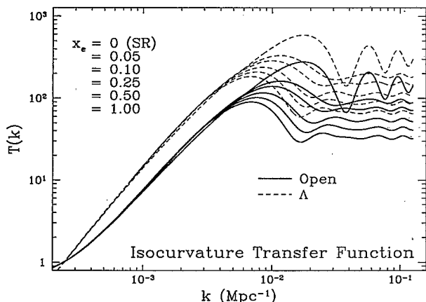
FIG. 17. The isocurvature matter transfer function ( \Omega_0 = 0.2 , h = 0.5 , numerical). The baryon perturbations will have a prominent peak at the maximal Jeans scale since perturbations grow as D(a) outside this scale, with a k^2 - 3K tail, and are suppressed inside it. The acoustic oscillations damp away in the highly ionized case since last scattering is delayed and the diffusion length grows. This leaves a flat small-scale tail in the transfer function. Note also that in the low ionization scenarios, the Jeans length may not grow to its maximum matter dominated value by last scattering, leading to a smaller scale for the peak. The growth suppression due to \Lambda is less significant than that from curvature domination.
