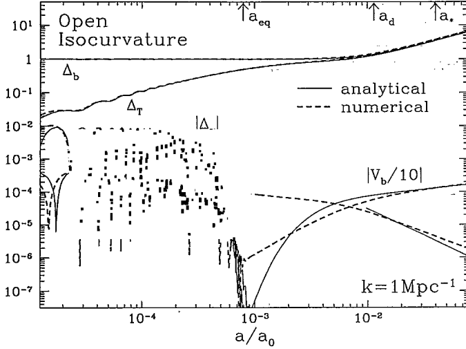
FIG. 10. Small-scale isocurvature evolution and photon diffusion ( \Omega_0 = 0.2 , h = 0.5 , no recombination). At small scales gravity may be ignored, yielding pure adiabatic oscillations. Perturbations in the photons damp once the diffusion length grows larger than the wavelength k_D < k . Likewise the adiabatic component of the baryon fluctuations also damps leaving them with the original entropy perturbation. After diffusion, the photons and baryons behave as separate fluids, allowing the baryons to grow once Compton drag becomes negligible a > a_d . Photon fluctuations are then regenerated by the Doppler effect as they diffuse across infalling baryons. The analytic approach for the photons in this limit applies between the drag epoch and last scattering a_d < a < a_* .
