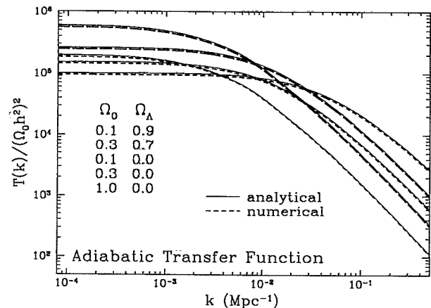
FIG. 16. The adiabatic matter transfer function ( h = 0.5 , \Omega_b = 0.01 ). The transfer function has been scaled by (\Omega_0 h^2)^{-2} to compare different \Omega_0 values by requiring the same initial gravitational potential \Phi (below the curvature scale). For scale invariant n = 1 \Lambda models, this normalization is equivalent to that determined by large-scale anisotropies, since the SW effect dominates all but the lowest multipoles. Therefore, the approximate relative amplitude of matter fluctuations can be directly read off from this plot. For open models, this is not true due to a more significant ISW effect and curvature effects at large scales which relate the potential to the initial power spectrum.
