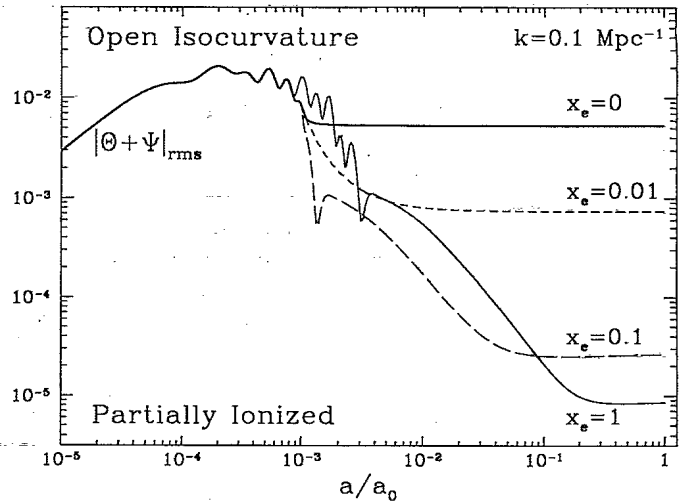
FIG. 15. Small-scale isocurvature temperature evolution under partial reionization ( \Omega_0 = 0.2 , h = 0.5 , numerical). If the Universe stays transparent after standard recombination at z_* \simeq 1000 , the acoustic oscillations in the photon fluid will be frozen. However these large fluctuations are suppressed by diffusion damping in partially reionized models. Although the Doppler and other diffusive effects regenerate fluctuations at small scales, these effects are also suppressed under the diffusion length (i.e., the thickness of the last scattering surface).
