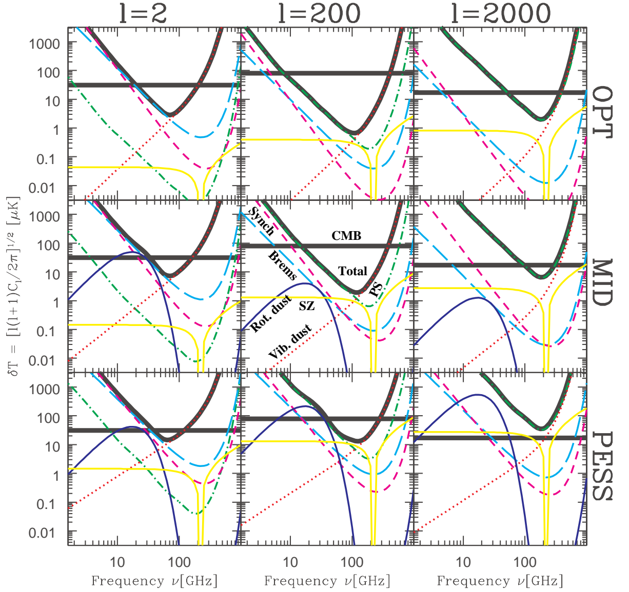
FIG. 8.— The frequency dependence of our unpolarized foregrounds is shown for three angular scales ( \ell = 2 , \ell = 200 and \ell = 2000 ) for the optimistic (OPT), middle-of-the-road (MID) and pessimistic (PESS) scenarios described in the text. The thin curves correspond to synchrotron radiation (short-dashed), free-free emission (long-dashed), spinning dust (solid), vibrational dust (dotted), point sources (dot-dashed) and SZ (solid grey/yellow). The thick curves show the CMB (horizontal line) and the total for all foregrounds.
