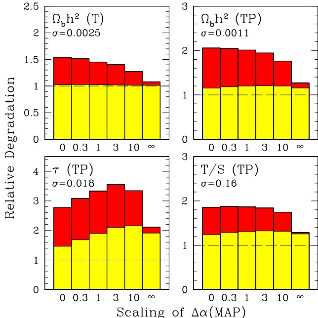
FIG. 22.— As Figure 18, but altering the frequency coherence \Delta\alpha of the fiducial foreground model. We scale all \Delta\alpha (see Table 2) by a factor of 0, 0.3, 1, 3, 10, and \infty . As shown in T98, perfect coherence and perfect decoherence are the best-cases; intermediate values yield worse performance. All errors are shown relative to those in the case with no foregrounds.
