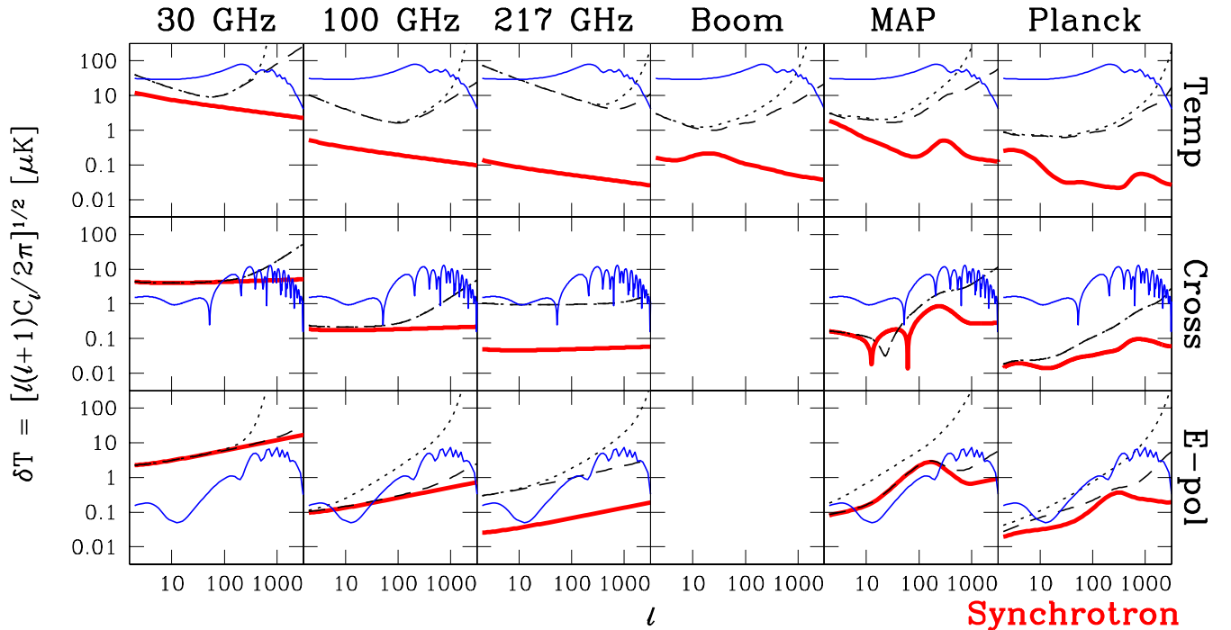
FIG. 1.— The MID model for synchrotron radiation (heavy line). The first three columns show the uncleaned amplitude as a function of scale at 30, 100 and 217 GHz. The rows show the temperature ( T ), cross-correlation ( X ) and E -channel polarization, respectively. For reference, the CMB power spectrum of our our fiducial \Lambda CDM cosmology (§ 5.1) is also shown (thin solid line) together with the total foreground power including (dotted) and excluding (dashed) Planck detector noise. The second three columns show the foregrounds amplitude when the maps are cleaned according to the optimal procedure in § 4; this method assumes that the foreground properties are well-known. The cleaning depends on the experimental specifications; we show results for Boomerang , MAP and Planck .
