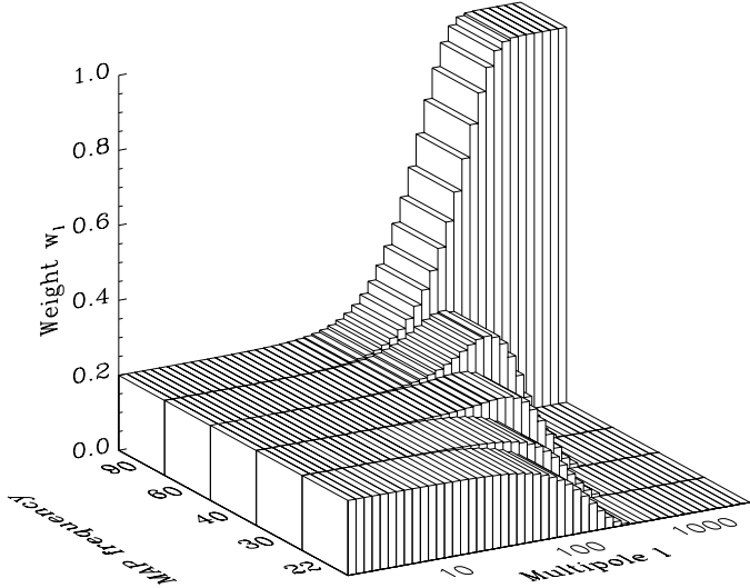
FIG. 9.— The weights w_\ell^T with which the 5 unpolarized MAP channels are combined into a single map are plotted as a function of angular scale \ell for the case of no foregrounds. Similar plots for the Wiener filtering method can be found in AAO (1998) and BG99.
