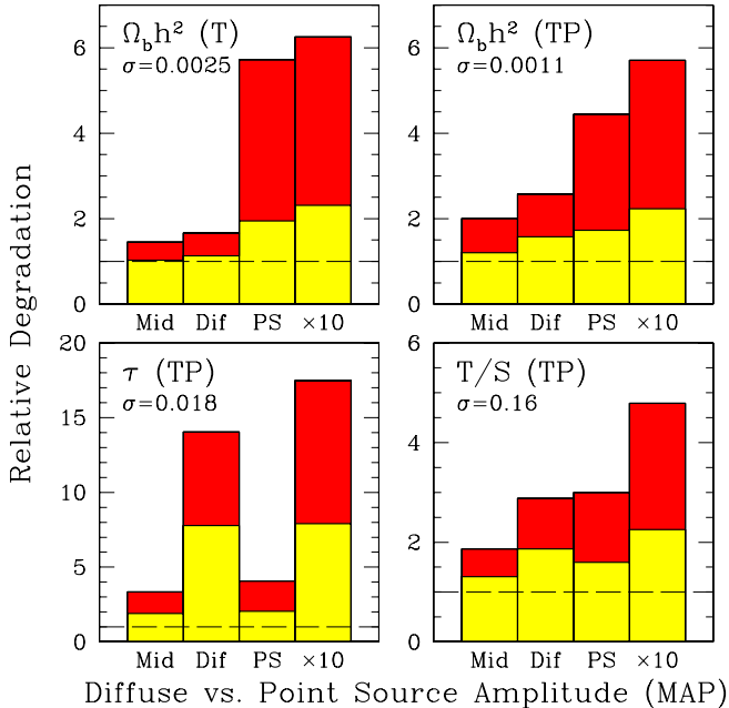
FIG. 20.— As Figure 18, but increasing the diffuse foregrounds and point sources separately. “Mid” bars refer to the MID foreground model, simultaneously estimating the foreground parameters. “Dif” bars show the results when the diffuse components (i.e. all those that are not point sources) are increased by 10 in amplitude. “PS” bars show the results when the point source and SZ components have their amplitude (after PSF fitting) increased by a factor of 10. “ \times 10 ” bars show the combined result. All values are shown as the fractional increase relative to the results with no foregrounds. This figure shows the case for MAP .
