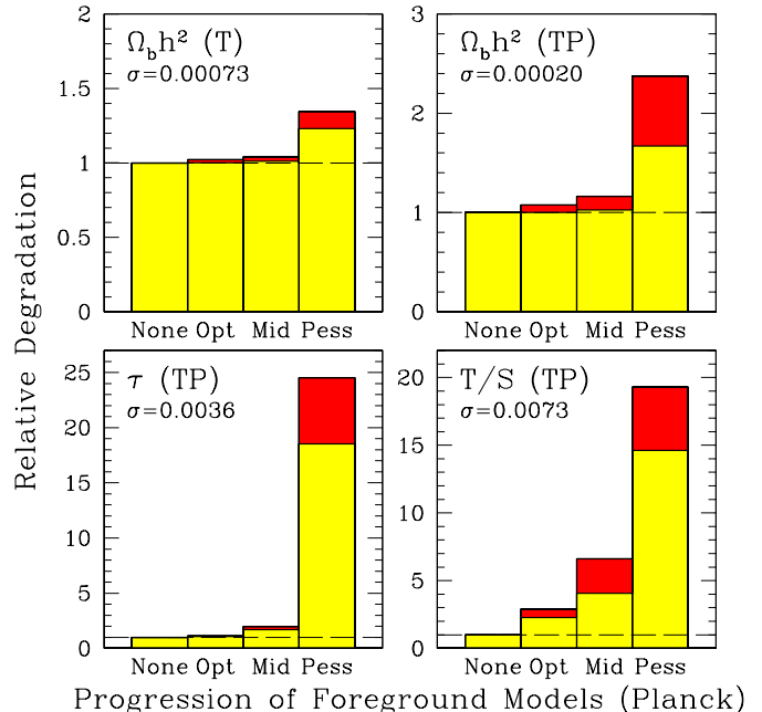
FIG. 19.— As Figure 18, but for Planck .
