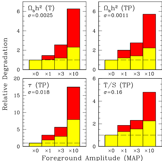
FIG. 25.— As Figure 18, but showing the relative degradation in error bars from MAP on four cosmological parameters as the amplitude of foregrounds are increased. The histograms show results for a series of foreground models based on our MID model, with amplitudes of all components multiplied by 0 (i.e. no foregrounds), 1, 3, and 10. The results are scaled to the no-foreground case; the 1 - \sigma errors in this case are listed in each panel. ( lightly-shaded ) Results with foregrounds of known properties. ( heavily-shaded ) Results with foregrounds with unknown parameters that must be simultaneously estimated from the CMB data.
