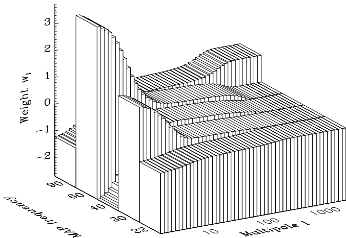
FIG. 10.— Same as Figure 9, but for the MID foreground scenario.
