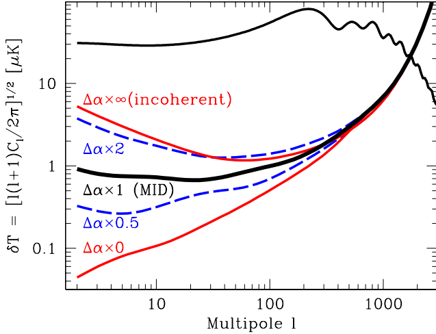
FIG. 12.— The effect of frequency coherence. The total power spectrum from noise and foregrounds in the cleaned Planck T map is shown for five different assumptions about frequency coherence, corresponding to multiplying all values of \Delta\alpha from the MID model (heavy curve) by \infty , 2, 1, 0.5 and 0, respectively (from top to bottom). The fiducial CMB power spectrum is shown for comparison.
