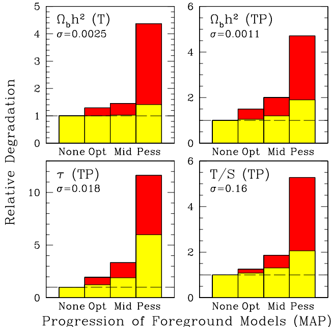
FIG. 18.— Relative degradation in error bars from MAP on four cosmological parameters as the amplitude of foregrounds are increased. ( top-left ) Behavior of \Omega_b h^2 with intensity information only (T). ( proceeding clockwise ) \Omega_b h^2 , T/S , and \tau with intensity and polarization information (TP). Bars show the error bar for each foreground case relative to the no-foregrounds case; the 1 - \sigma error of the latter is listed in each panel. The histograms show results for a series of foreground models, ranging from no foregrounds to our OPT, MID, and PESS models. ( lightly-shaded ) Results with foregrounds of known properties. ( heavily-shaded ) Results with foregrounds whose parameters must be simultaneously estimated from the CMB data.
