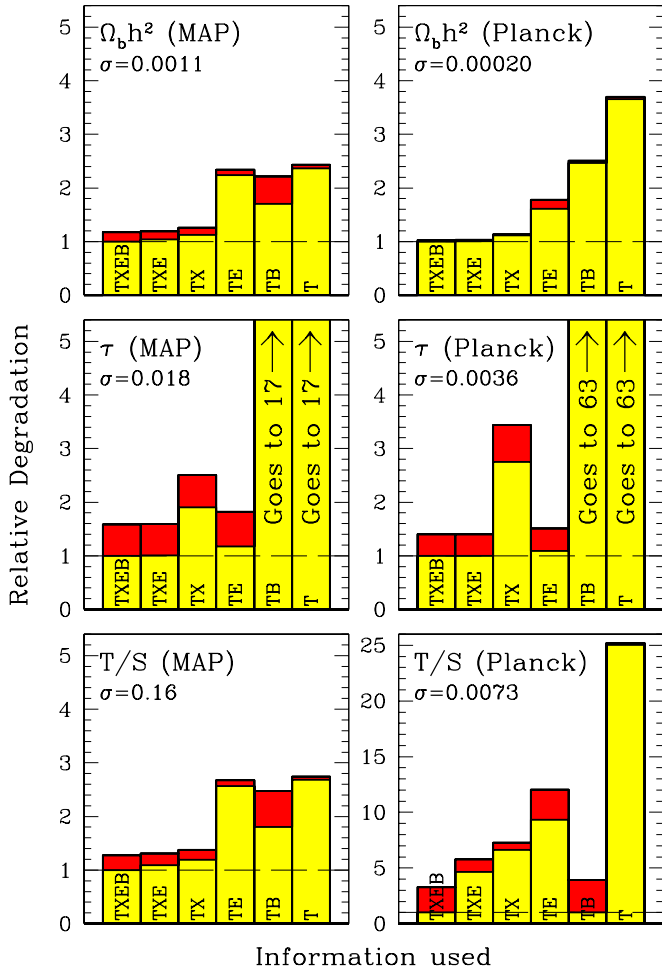
FIG. 24.— Information about cosmological parameters from different polarization types. In each panel, the bars show the relative error bars using all information ( TXEB ), all but B -polarization ( TXE ), T and X only ( TX ), T and E only ( TE ) and unpolarized intensity alone ( T ). Results are shown both without any foregrounds (yellow) and for the MID foreground scenario with known properties (red). Note that these color conventions differ from those in Figure 18–23 and 25 and also that this figure uses a Gaussian rather than exponential coherence function. The rightmost bars in the \tau panels extend far off the scale.
