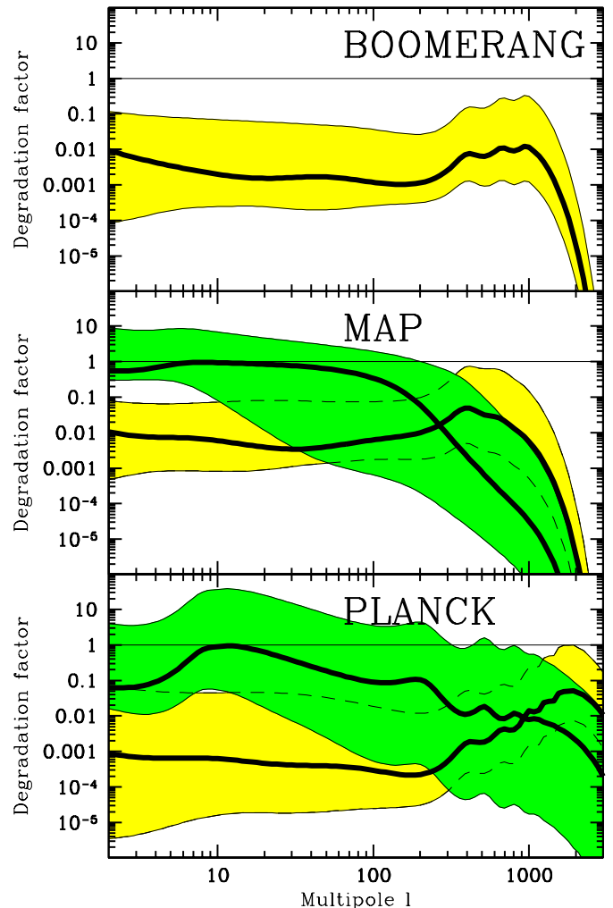
FIG. 11.— Degradation factors. The fraction \text{DF} - 1 by which foregrounds increase the power spectrum error bars is shown for Boomerang (top), MAP (middle) and Planck (bottom). Each shaded band shows the range of uncertainty between the PESS and OPT models, with the MID case indicated by a heavy curve. The lighter band is for intensity T , the darker one for E polarization.
