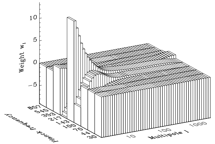
FIG. 14.— The weights \mathbf{w}_\ell^T with which the unpolarized maps at the 9 Planck frequencies are combined into a single map are plotted as a function of angular scale \ell for the MID foreground model.
