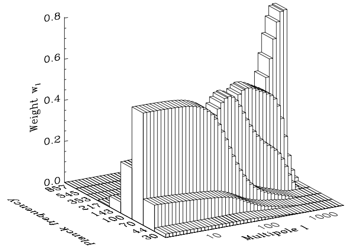
FIG. 13.— The weights \mathbf{w}_\ell^T with which the unpolarized maps at the 9 Planck frequencies are combined into a single map are plotted as a function of angular scale \ell for the MID model, but with completely incoherent foregrounds ( \Delta\alpha = \infty ).
