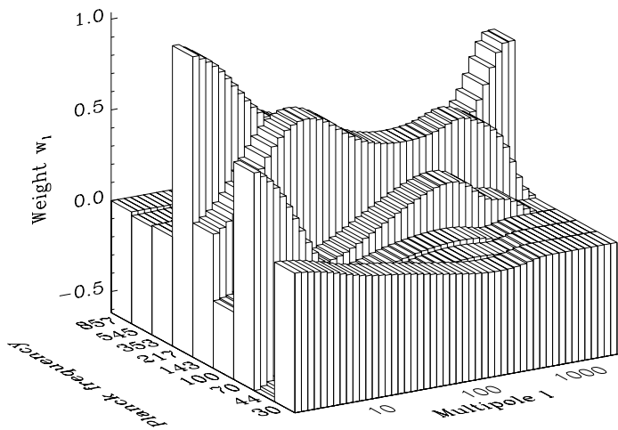
FIG. 15.— The weights w_\ell^T with which the unpolarized maps at the 9 Planck frequencies are combined into a single map are plotted as a function of angular scale \ell for the MID model, but with perfectly coherent foregrounds ( \Delta\alpha = 0 ).
