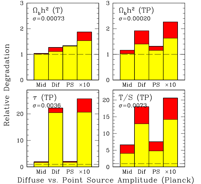
FIG. 21.— As Figure 20, but for Planck .
