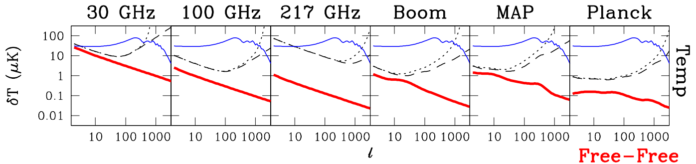
FIG. 2.— Same as Fig. 1, but for free-free emission.
