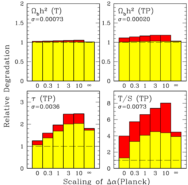
FIG. 23.— As Figure 22, but for Planck .
