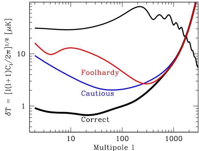
FIG. 16.— The effect of faulty assumptions about frequency coherence. The total power spectrum from noise and foregrounds in the cleaned Planck T map is shown for the MID model using three different assumptions for the cleaning process: the correct (MID) \Delta\alpha -values (bottom), \Delta\alpha = \infty (middle, cautious) and \Delta\alpha = 0 (top, foolhardy). The fiducial CMB power spectrum is shown for comparison.
