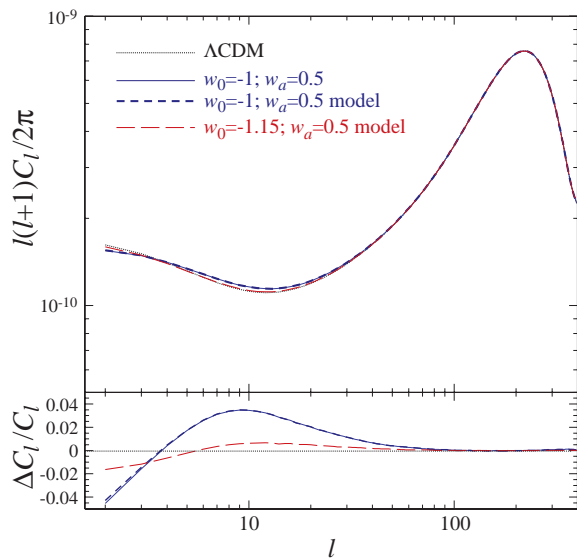
FIG. 2: Model predictions for the CMB anisotropy power spectrum relative to a fiducial \Lambda CDM model. For models that do not cross the phantom divide, e.g. w_0 = -1 , w = 0.5 , the 2 field model matches the single field predictions to 0.1%. For crossing models that mimic a cosmological constant by having w_n \approx -1 , e.g. w_0 = -1.15 , w = 0.5 , the deviations are essentially indistinguishable.
