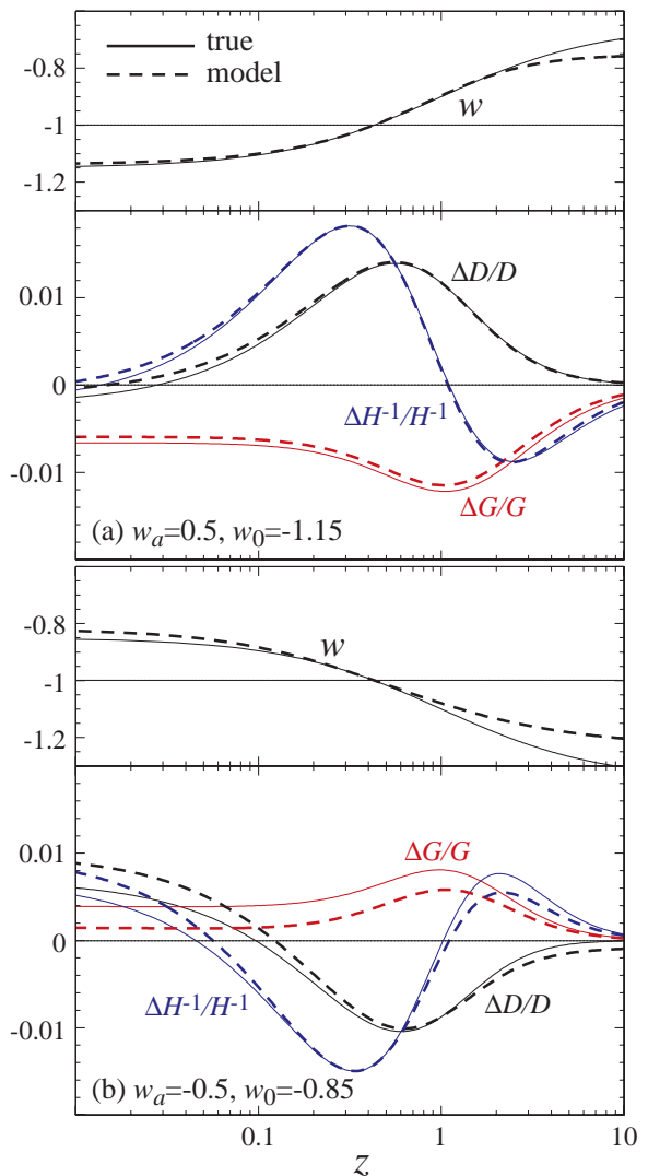
FIG. 1: Target versus 2 field model behavior of w and the dark energy observables relative to a fiducial \Lambda model (dotted line, see text). Even in this nearly worst case scenario where w crosses the phantom divide near the pivot point a \sim 3/4 or z \sim 0.3 , the model reproduces the observables to 0.1% accuracy for w_a > 0 and only a factor of a few larger for w_a < 0 .
