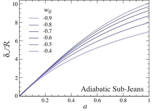
FIG. 1. Adiabatic matter density perturbation evolution \delta relative to the initial curvature fluctuation \mathcal{R} for an arbitrary wavenumber on sub Jeans scales. Pressure support in the scalar field Q slows the growth of fluctuations as w_Q increases and dark energy domination occurs earlier. Here and throughout the figures, we take \Omega_m = 1 - \Omega_Q = 0.3 .
