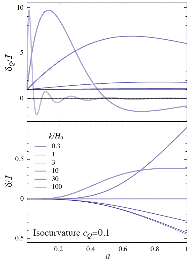
FIG. 4. Growth of the dark energy and matter density perturbations \delta_Q and \delta from dark energy isocurvature initial conditions \mathcal{I} for c_Q = 0.1 . Dark energy perturbations (top) are frozen outside the horizon k/H_0 < 1 , grow between the horizon and sound horizon, and oscillate below the sound horizon. Matter perturbations (bottom) are anticorrelated with \mathcal{I} outside the horizon, grow in correlation with it between the horizon and sound horizon, and are independent of it below the sound horizon. By adding isocurvature modes to the adiabatic modes, the separate universe construction and observable response can depend on scale even for w_Q \approx -1 .
