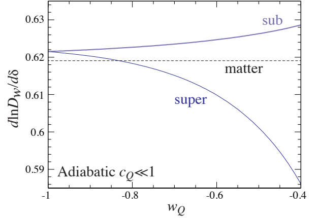
FIG. 3. Response of the short wavelength linear growth function D_W to the long wavelength density field \delta at a = 1 for adiabatic initial conditions and scalar field dark energy with c_Q \ll 1 . This response depends on whether the long wavelength is super or sub Jeans scale. Long wavelength scale dependence of the squeezed bispectrum and trispectrum would result but vanishes if w_Q \rightarrow -1 . For reference, the second order response in the matter dominated regime 13/21 is also shown (dashed).
