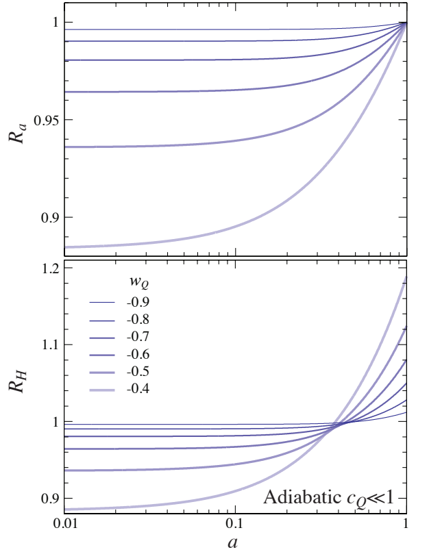
FIG. 2. Ratios of super to sub Jeans scale separate universe changes in the scale factor \delta \ln a (top) and Hubble rate \delta \ln H (bottom) for the same long wavelength density \delta_0 today. Above the Jeans scale, the scale factor is always closer to global whereas the Hubble rate is closer at early times and further at late times. Observable responses to \delta_0 therefore depend on its scale, but as w_Q \rightarrow -1 this difference vanishes. Here initial conditions are adiabatic and c_Q \ll 1 .
