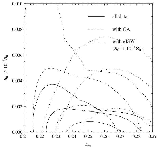
FIG. 6: Contours of 2D marginalized 68%, 95%, and 99% confidence boundaries using WMAP5, ACBAR, CBI, VSA, Union, SHOES, and BAO in combination with the additional data sets. For gISW, the Compton wavelength is rescaled as B_0 \rightarrow 10^{-2}B_0 , i.e., the constraint is a factor of 10^2 weaker than illustrated. gISW cross correlations favor higher values of \Omega_m and break the degeneracy between \Omega_m and B_0 seen in the CA data.
