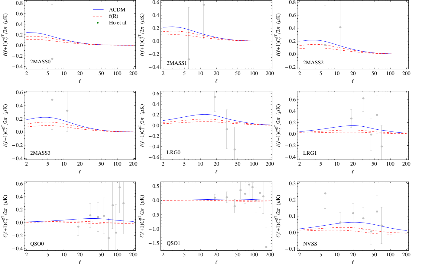
FIG. 2: Best-fit \Lambda CDM ( B_0 = 0 ) gISW cross correlations (blue solid line) for the different galaxy samples, roughly ordered in increasing effective, bias-weighted, redshift. Adding non-zero values for the Compton wavelength parameter (red dashed lines): B_0 = 0.1 (top) and B_0 = 0.5 (bottom).
