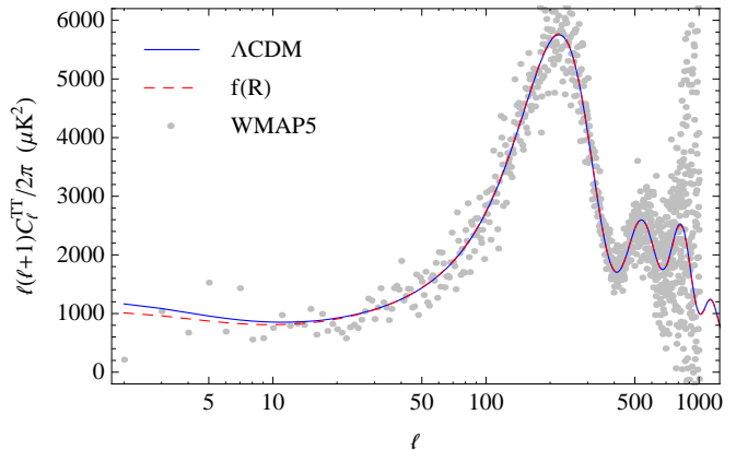
FIG. 1: Best-fit CMB temperature anisotropy power spectrum for \Lambda CDM and f(R) gravity from using the Union, SHOES, BAO, and CMB data.
