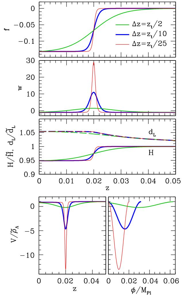
FIG. 1: Hubble transitions with different redshift widths corresponding to the potential-dominated model of Eqs. (8) and (10): \Delta z = z_t/2 (medium thickness, green), z_t/10 (thick, blue), and z_t/25 (thin, red). All models have a transition at z_t = 0.02 with amplitude \delta = -0.05 and tildes denote the \Lambda CDM reference model with \tilde{\Omega}_m = 0.24 , \tilde{\Omega}_\Lambda = 0.76 , and \tilde{h} = 0.73 . Upper panels: redshift evolution of various observables. Lower panels: scalar field model potential.
