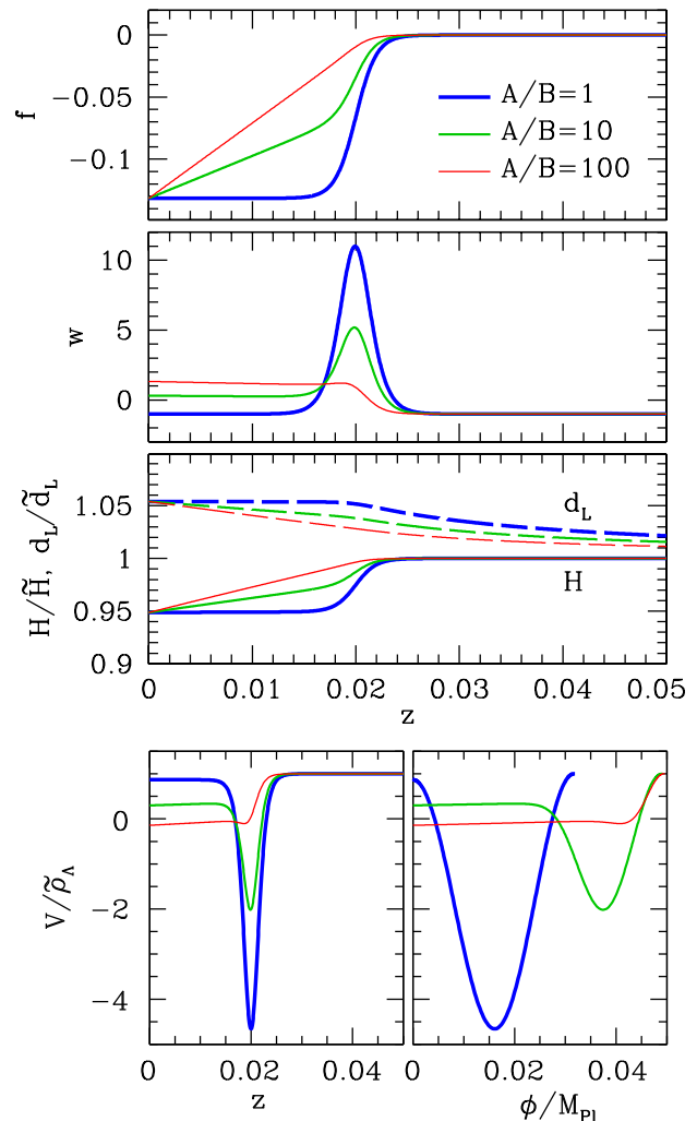
FIG. 2: Hubble transitions with different ratios of potential to kinetic energy at z = 0 , using the generalized model of Eqs. (11) and (12) with A/B = 1 ( thick, blue ), 10 ( medium thickness, green ), and 100 ( thin, red ). The A/B = 1 model corresponds to zero kinetic energy after the transition as in Fig. 1, and A/B \rightarrow \infty to maximal kinetic energy. All models have z_t = 0.02 of width \Delta z = z_t/10 and amplitude \delta = -0.05 .
