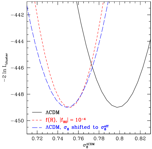
FIG. 3: Cluster likelihood as function of primordial normalization (quantified by the linear power spectrum normalization \sigma_8^{\Lambda\text{CDM}} a \Lambda\text{CDM} model would give), for fixed values of \Omega_m = 0.258 , h = 0.716 , and |f_{R0}| = 10^{-4} in case of the f(R) prediction. The red short-dashed line shows the likelihood calculated using the full f(R) mass function enhancement, while the blue long-dashed line shows the \Lambda\text{CDM} likelihood obtained with the rescaled normalization, \sigma_8^{\text{eff}} .
