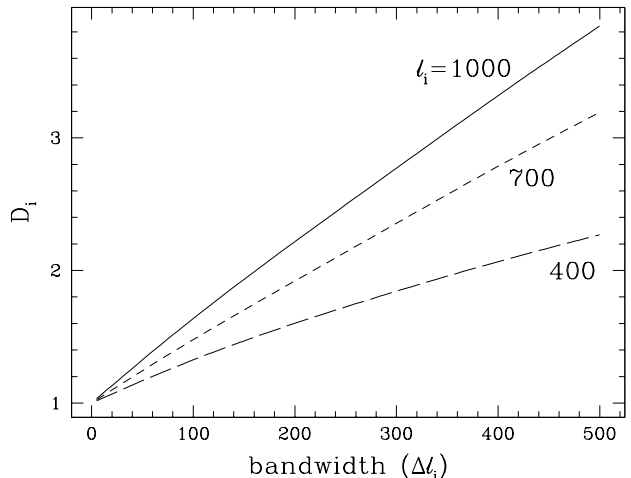
FIG. 3: Bandpower variance degradation factor D_i as a function of bandwidth for various choices of the central l_i of the band. The degradation increases with the bandwidth since the Gaussian contribution decreases with the number of wave-modes. The trend illustrates the effect of the non-Gaussian correlation.
