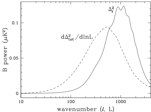
FIG. 1: B power spectrum \Delta_l^2 = l^2 C_l^{BB} / 2\pi and the differential contribution to the total B variance \Delta_{\text{tot}}^2 from power in the lensing field \phi with wavenumber L [see Eqn. (9)]. Even though the B power peaks at l \sim 10^3 , it gains half its contribution from power in the lensing field at L \lesssim 450 . Sampling errors in B therefore reflect the larger scale variations in \phi .
